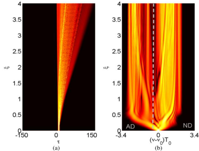
Fig. 5. (a) Temporal and (b) spectral evolution under conditions identical to those of Fig. 1 except that the sign of TOD is reversed ( \delta_3 = 0.05 ).
