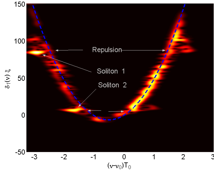
Fig. 8. Spectrogram at a distance \xi = 2 for N = 10 and \delta_3 = 0.05 . The dotted curve represents the delay.
