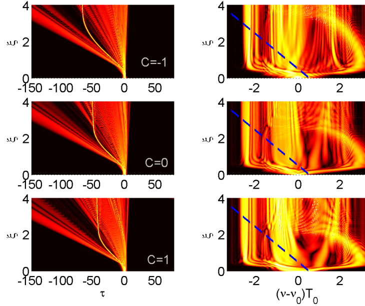
Fig. 9. Temporal (left column) and spectral (right column) evolution under conditions identical to those used in Fig. 1 except that the chirp parameter takes values from -1 to 1 . The blue dotted lines show \delta_2 as function of normalized frequency.
