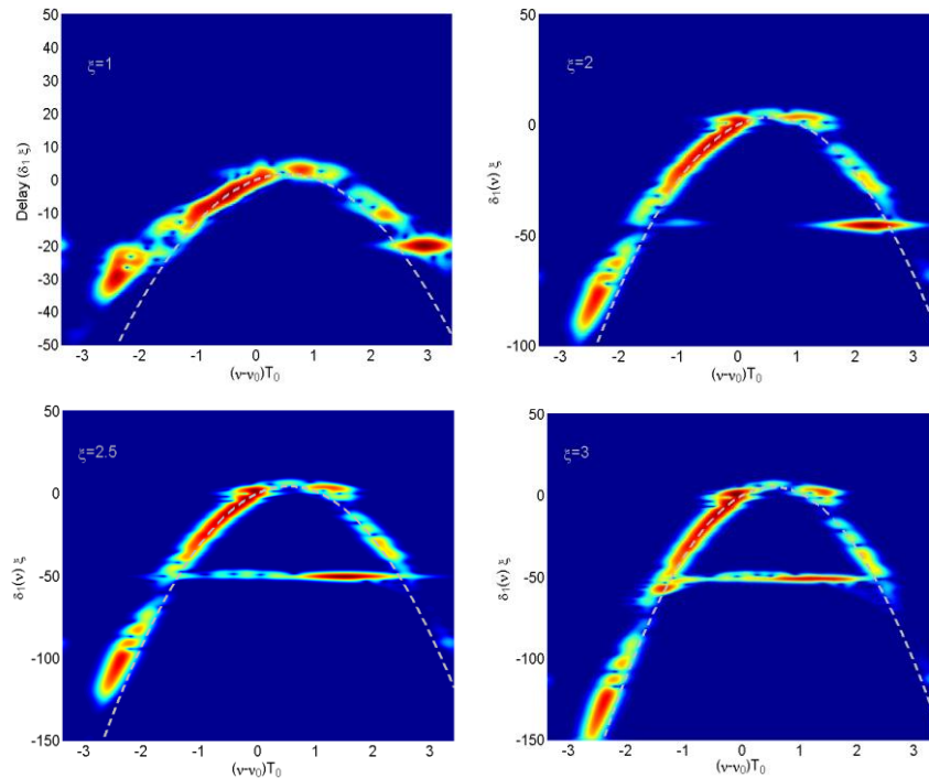
Fig. 3. Spectrograms of the pulse at four different lengths for parameter values identical to those used in Fig. 1. The dotted curves represent the time delay ( \delta_l \xi ).
