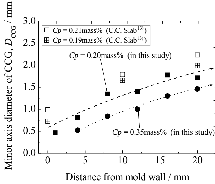
Fig. 4. Relationship between the minor axis diameter, D_{CCG} , and the distance from mold wall in 0.2C and 0.35C samples. Also, the corresponding data for the C.C. slab [13] are plotted for comparison.
