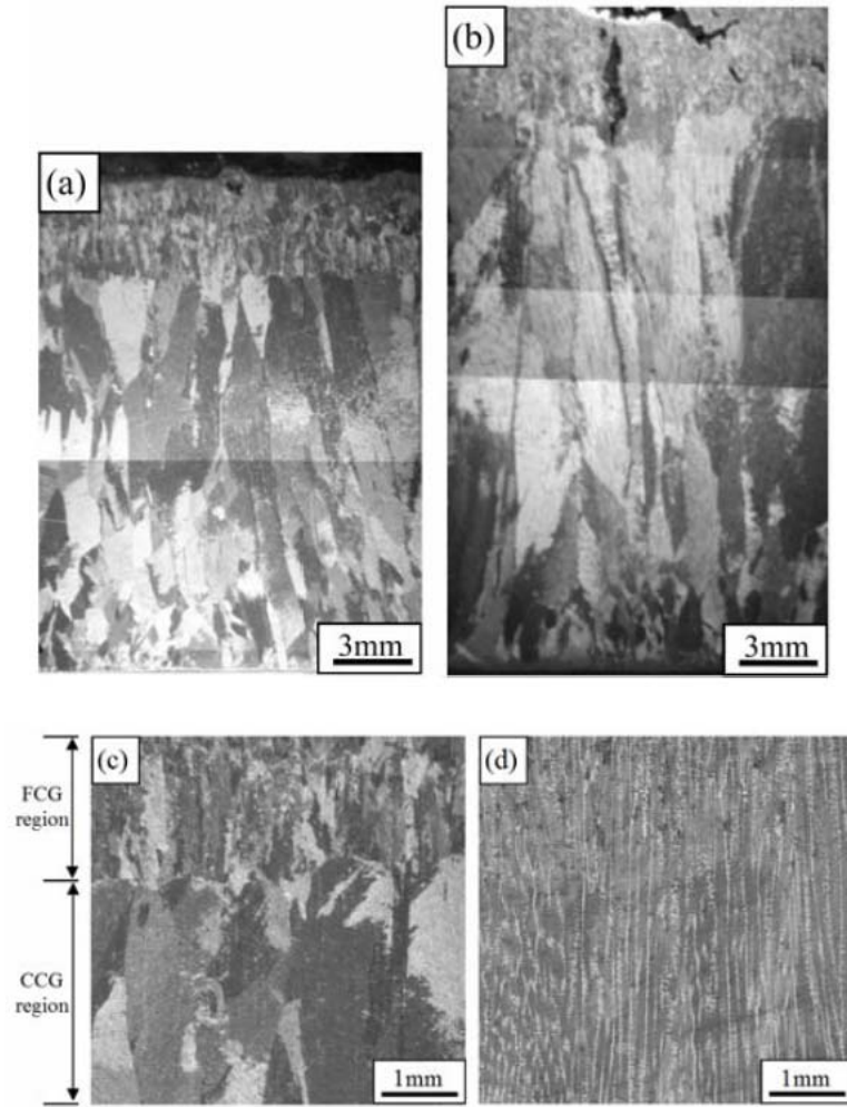
Fig. 5. Micrographs of the structures in 0.2C sample quenched at different times. As-cast \gamma structure in 0.2C sample quenched at (a)30s, (b)50s. (c) Enlargement of the FCG/CCG region boundary in 0.2C sample quenched at 30s. (d) Dendrite structure in the same region as in Fig. 5(c). The bottom side and the upper side correspond to the mold side and the upper side of the ingot, respectively.
