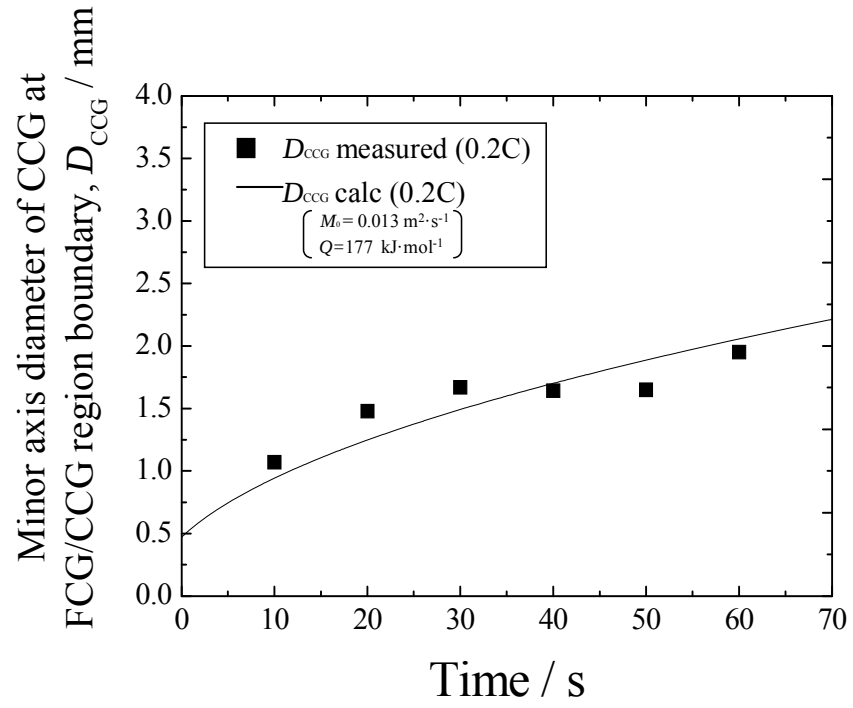
Fig. 8. Relationship between D_{\text{CCG}} at the FCG/CCG region boundary and the time after casting. Solid line was calculated from equation (1).
