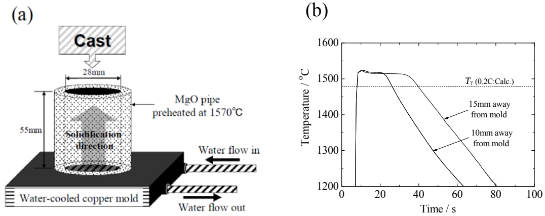
Fig. 2. (a) Schematic illustration of the rapid unidirectional solidification equipment used in this study. (b) Cooling curves monitored in the 0.2C sample at 10 and 15mm heights from the copper mold.
