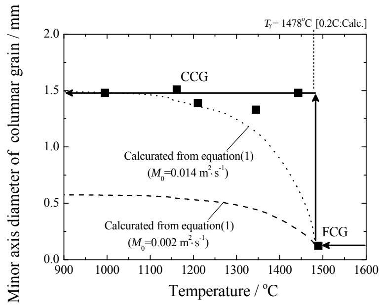
Fig. 7. Comparison of the \gamma grain growth behavior at a position in 0.2C steel 8mm away from mold with those calculated from the equation (1).
