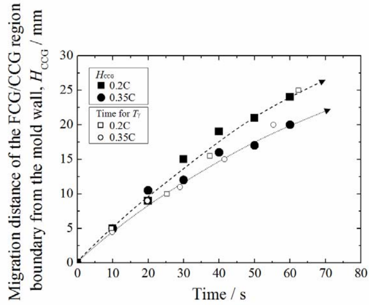
Fig. 6. Relationship between H_{CCG} and the holding time in 0.2C and 0.35C samples. The open marks indicate the time when the temperature reaches T_\gamma in the cooling curve at each position.
