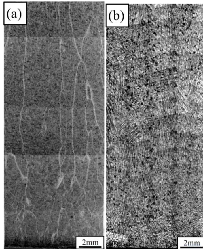
Fig. 3. Micrographs of the 0.2C sample naturally cooled to RT showing (a) as-cast \gamma structure and (b) dendrite structure. The bottom side and the upper side correspond to the mold side and the upper side of the ingot, respectively. The bright boundaries in Fig. 3(a) represent the as-cast \gamma grain boundaries. These boundaries are visible because of the primary ferrite phase precipitating on the \gamma grain boundary.
