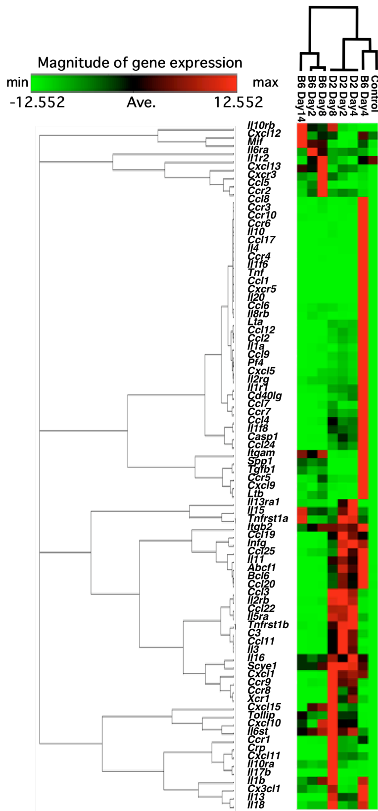
Fig 2.1. Cluster analysis showing heat map of mouse inflammatory cytokine/chemokine and receptor genes regulated in lungs of B6, D2 and control mice. A 2D gene tree was created using the average linkage clustering heat map method. Genes with a change in fold ( P < 0.001 ) are depicted. Each row represents lung of each mouse group at indicated time points and the hierarchical structure of the time-points and infections is illustrated as a dendrogram while the fold change values are color encoded with green for down-regulated genes, black for average unregulated genes and red for up-regulated genes.
