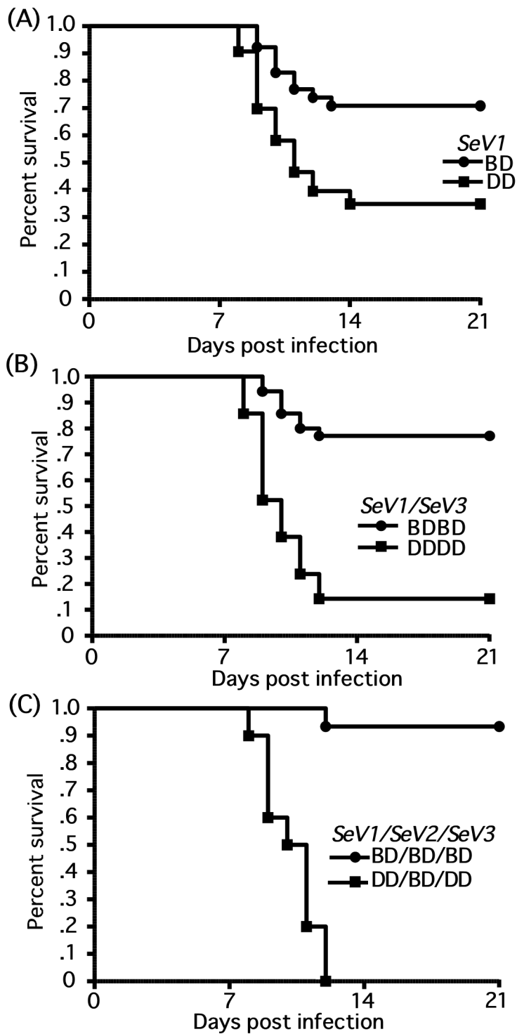
Fig. 1.7. Kaplan–Meier plot of SeV-infected backcrossed mice with respect to their genotypes of SeV1 , SeV2 , and SeV3 loci. (A) Kaplan–Meier plot of mice possessing heterozygous or homozygous with respect to SeV1 . (B) Kaplan–Meier plot of mice with respect to SeV1 and SeV3 . (C), Kaplan–Meier plot of mice with respect to SeV1 , SeV2 , and SeV3 . In this analysis, SeV2 (D3Mit182) is fixed to heterozygous to show epistatic interaction. In (A), (B), and (C), the survival rate was determined as the rate of mice showing less than 40% body weight loss after SeV infection in the light of “humane endpoint” concept.
