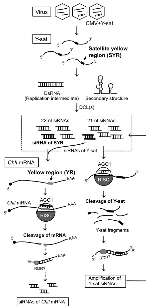
Figure 7. Scenarios to explain the cleavage of ChlI mRNA by Y-sat in the RNA silencing pathway. The most probable scenario is that AGO1 associated with the primary Y-sat siRNAs cleaves the ChlI mRNA at the SYR-YR portion, then a host RNA-dependent RNA polymerase (RDR) may access the cleaved ChlI mRNA fragments to produce dsRNAs, which are subsequently processed into secondary siRNAs. In addition, Y-sat itself is cleaved by AGO1 loaded with siRNAs derived from Y-sat, inducing the production of a large amount of siRNAs containing the SYR sequence. doi:10.1371/journal.ppat.1002021.g007
