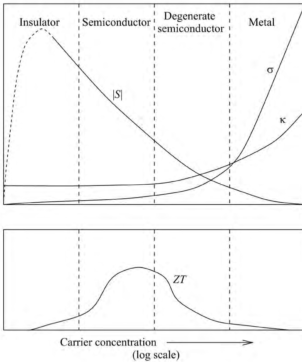
Figure 1-5: What materials can have high ZT ?
