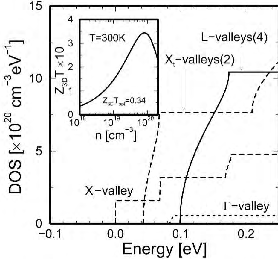
Figure 4-13: Density of states for electrons (DOS) for a (001) oriented GaAs(20 Å)/AlAs(30 Å) superlattice calculated for various subbands derived from \Gamma -, X_l -, X_t - and L -valleys, as indicated in the figure. The number inside the parentheses denotes the number of equivalent valleys that are degenerate in energy. Therefore, the DOS for X_t -valleys shown here, for example, includes contributions from two equivalent X_t -valleys. The inset shows a plot for the calculated Z_{3D}T as a function of carrier concentration n for this superlattice at 300 K. The position of the chemical potential \zeta that gives the optimum value of Z_{3D}T (denoted as Z_{3D}T_{opt} ) is \zeta = 0.107 eV on the main scale.
