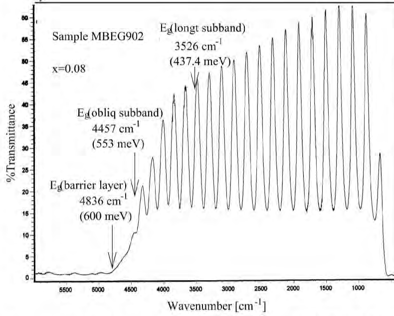
Figure B-5: IR transmission spectrum for a (111) oriented PbTe(20 Å)/Pb 1-x Eu x Te(400 Å) multiple-quantum-well sample (MBEG902). The values of the optical energy band gaps given in the figure are obtained by the Krönig-Penney model using Eqs. B.12 and B.13 to calculate the conduction and valence band offsets at T = 300 K, where the value of x (Eu content) used in the calculation is also given in the figure ( x = 0.08 ).
