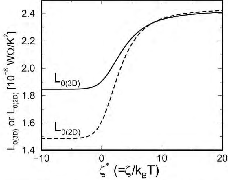
Figure 2-8: Lorenz number L_{0(3D)} (solid curve) and L_{0(2D)} (dashed curve) defined by Eqs. 2.13 and 2.22, respectively, as a function of reduced chemical potential \zeta^* (= \zeta/k_B T) . L_{0(3D)} and L_{0(2D)} approach the traditional value for metals at large \zeta^* .
