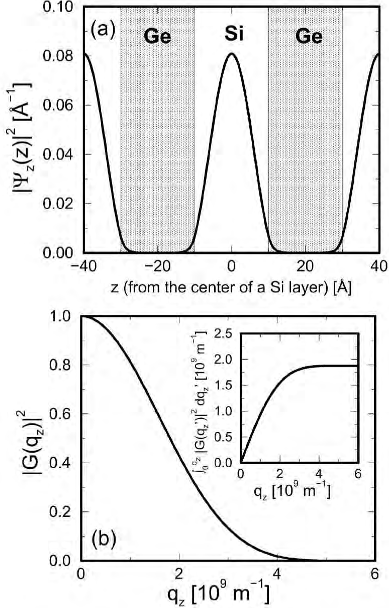
Figure 6-1: (a) Squared wavefunction |\psi_z(z)|^2 for a (001) oriented Si(20 \text{\AA} )/Ge(20 \text{\AA} ) superlattice [ \Delta_{\parallel} -subband in Fig. 5-8(a)] as a function of z , which is used for the calculation of G(q_z) (the Fourier transform of |\psi_z(z)|^2 ) in (b). \psi_z(z) is obtained by solving the Schrödinger equation using the Krönig-Penney model as discussed in §4.3.4. The calculation was made using the value of the conduction band offset \Delta E_c = 0.808 eV and the value of the z component (along the superlattice growth axis) of the effective mass tensor m_z = 0.92m (for both Si and Ge layers). (b) |G(q_z)|^2 as a function of q_z , where G(q_z) is defined in Eq. 3.7, for the wavefunction given in (a). The inset shows the integration of |G(q'_z)|^2 with respect to q'_z from zero to q_z as a function of q_z . Note that such a factor (with q_z = \infty ) appears in the squared matrix element for longitudinal acoustic phonon deformation potential scattering without including the effect of the free carrier screening (see Eq. 3.14).
