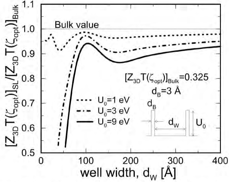
Figure 7-4: Plot of the calculated thermoelectric figure of merit Z_{3D}T at the optimum carrier concentration at 300 K for (111) oriented PbTe-based superlattices (normalized by the corresponding value for bulk PbTe) as a function of the quantum well width d_W . In obtaining these results, a relatively small value for d_B (barrier layer thickness) [ d_B = 3 \text{ \AA} ], and relatively large values of the potential barrier height U_0 ( U_0 = 1, 3 , and 9 \text{ eV} ) are utilized to simulate the effect of the extra Te layers in the PbTe/Te superlattice. The calculated values for these (111) oriented PbTe-based superlattices are found to be reduced relative to the corresponding value for bulk PbTe, due to the lifting of the valley degeneracy [22] (see text and Chapter 2 for more discussion), which contradicts the experimental observation in §7.1.
