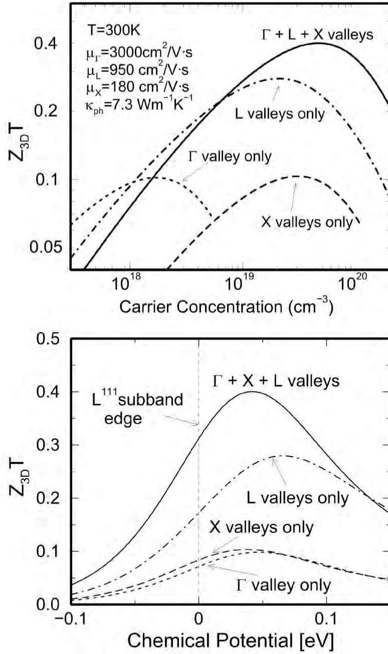
Figure 4-19: (a) Calculated Z_{3D}T s for a (111) oriented GaAs(20 Å)/AlAs(20 Å) superlattice as a function of carrier concentration treating \Gamma - (short-dashed curve), L - (dash-dotted curve) and X -valleys (long-dashed curve), separately, as well as treating all three types of valleys together (solid curve). (b) Calculated Z_{3D}T s for a (111) oriented GaAs(20 Å)/AlAs(20 Å) superlattice as a function of chemical potential measured from the longitudinal L -valley subband edge (the lowest conduction subband in energy) treating \Gamma - (short-dashed curve), L - (dash-dotted curve) and X - (long-dashed curve) valleys separately, as well as treating all three types of valleys together (solid curve).
