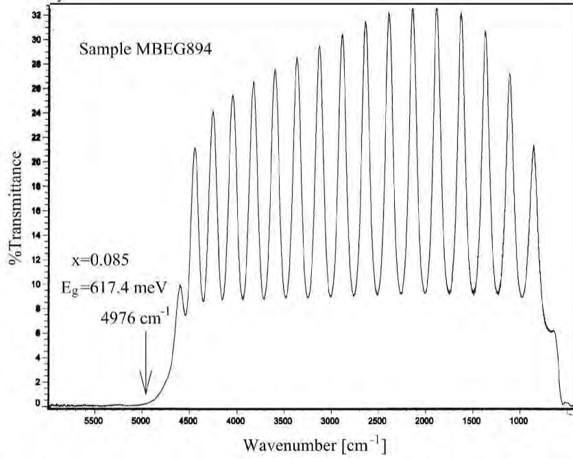
Figure B-4: IR transmission spectrum for a MBE-grown bulk (thick) \text{Pb}_{1-x}\text{Eu}_x\text{Te} film ( x \approx 0.08 ) sample (sample MBEG894). The value for the direct energy band gap shown in the figure ( E_g = 617.4 meV) is obtained for x = 0.085 and T = 300 K using Eq. B.12.
