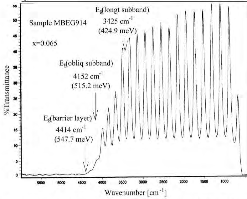
Figure B-9: IR transmission spectrum for a (111) oriented PbTe(20 Å)/Pb 1-x Eu x Te(400 Å) multiple-quantum-well sample (MBEG914). The values of the optical energy band gaps given in the figure are obtained by the Krönig-Penney model using Eqs. B.12 and B.13 to calculate the conduction and valence band offsets at T = 300 K, where the value of x (Eu content) used in the calculation is also given in the figure ( x = 0.065 ).
