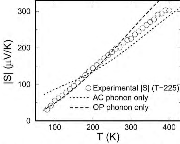
Figure 3-5: Absolute value of the Seebeck coefficient for the PbTe/Pb 1-x Eu x Te MQW sample (T-225) as a function of temperature (open circles) together with the theoretical results (1) considering only longitudinal acoustic phonon deformation potential scattering (short-dashed curve) and (2) considering only polar optic phonon scattering (long-dashed curve).
