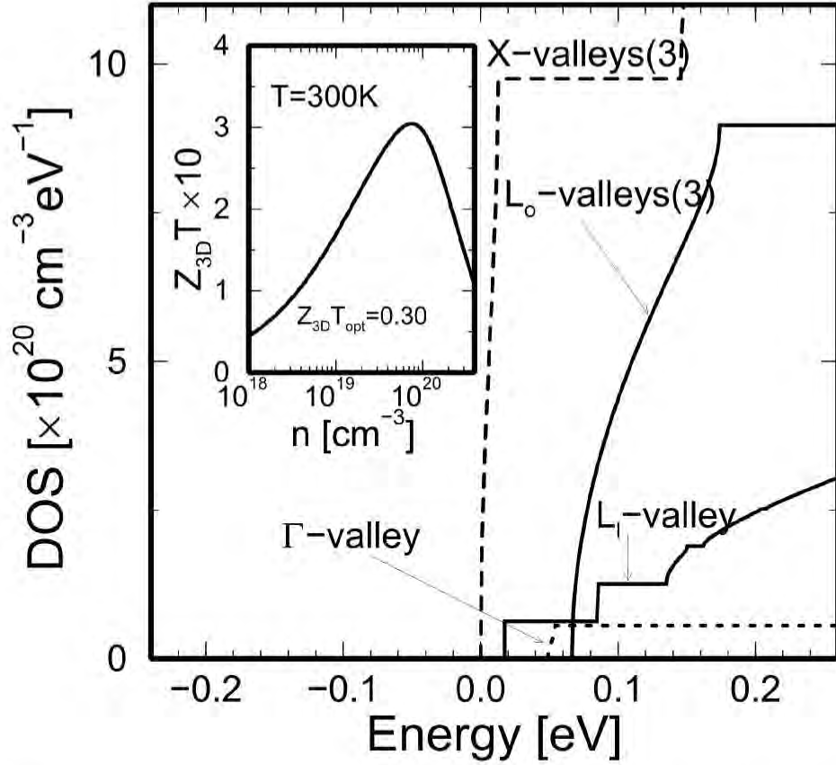
Figure 4-17: Density of states for electrons (DOS) for a (111) oriented GaAs(20 Å)/AlAs(30 Å) superlattice calculated for various subbands derived from \Gamma -, X -, L_v - and L_o -valleys, as indicated in the figure. The number inside the parentheses denotes the number of equivalent valleys that are degenerate in energy. Therefore, the DOS for L_o -valleys shown here, for example, includes contributions from three equivalent L_o -valleys. The inset shows a plot for the calculated Z_{3D}T as a function of carrier concentration n for this superlattice at 300 K. The position of the chemical potential \zeta that gives the optimum value of Z_{3D}T (denoted as Z_{3D}T_{opt} ) is \zeta = 0.067 eV on the main scale.
