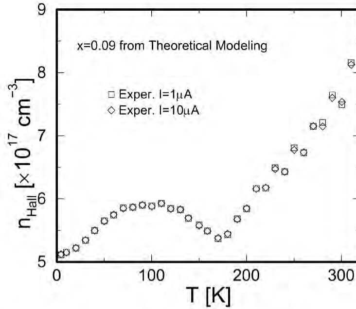
Figure B-18: Hall carrier density as a function of temperature for a (111) oriented \text{PbTe}(20 \text{ \AA})/\text{Pb}_{1-x}\text{Eu}_x\text{Te}(400 \text{ \AA}) multiple-quantum-well sample (MBEG909).
