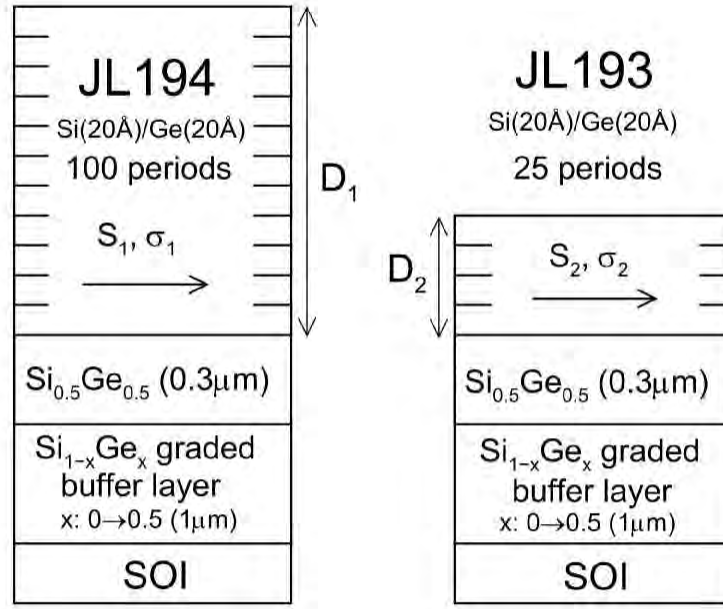
Figure 5-27: Schematic diagram to show the structures of the thin (25 periods) and thick (100 periods) Si(20 Å)/Ge(20 Å) superlattice samples that are used in the present investigation, which are denoted as JL193 and JL194, respectively.
