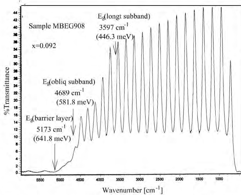
Figure B-6: IR transmission spectrum for a (111) oriented PbTe(20 Å)/Pb 1-x Eu x Te(400 Å) multiple-quantum-well sample (MBEG908). The values of the optical energy band gaps given in the figure are obtained by the Krönig-Penney model using Eqs. B.12 and B.13 to calculate the conduction and valence band offsets at T = 300 K, where the value of x (Eu content) used in the calculation is also given in the figure ( x = 0.092 ).
