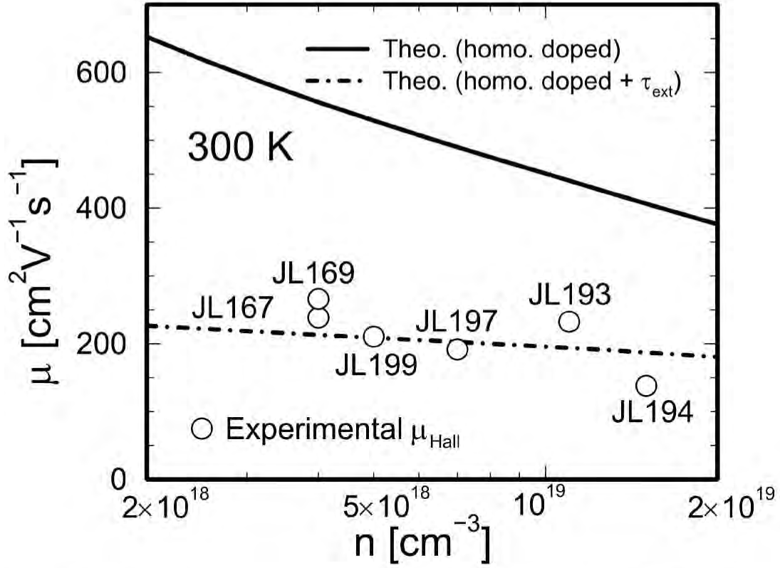
Figure 5-34: Experimentally determined Hall carrier mobility for the (001) oriented Si(20 Å)/Ge(20 Å) superlattices (open circles), that are obtained in §5.6–§5.8, as a function of Hall carrier concentration at 300 K. Also shown in the figure are the theoretically predicated carrier mobilities at 300 K for homogeneously doped (001) oriented Si(20 Å)/Ge(20 Å) superlattices using the semi-classical models developed in Chapter 6 without the use of any fitting parameters (solid curve), and using Matthiessen's rule (Eq. 5.6) to take into account the extrinsic scattering mechanisms that are discussed in §5.6.1 (dot-dashed curve), where a value of \tau_{\text{ext}} = 4 \times 10^{-14} s is chosen from Table 5.4 for the calculation of the theoretical carrier mobilities shown by the dot-dashed curve in the figure.
