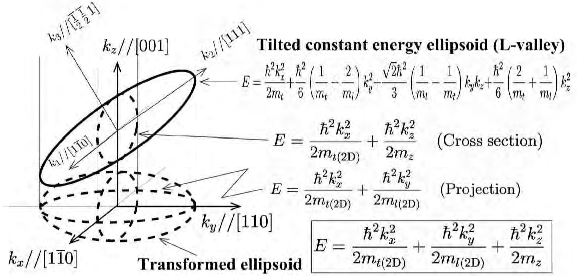
Figure 4-7: Schematic diagram to show how to construct the projected components [m_{t(2D)} and m_{l(2D)}] and the cross-sectional component ( m_z ) for the effective mass tensor \mathbf{M} for the L -point valley along the [111] direction in the Brillouin zone in (001) oriented GaAs/AlAs superlattices.
