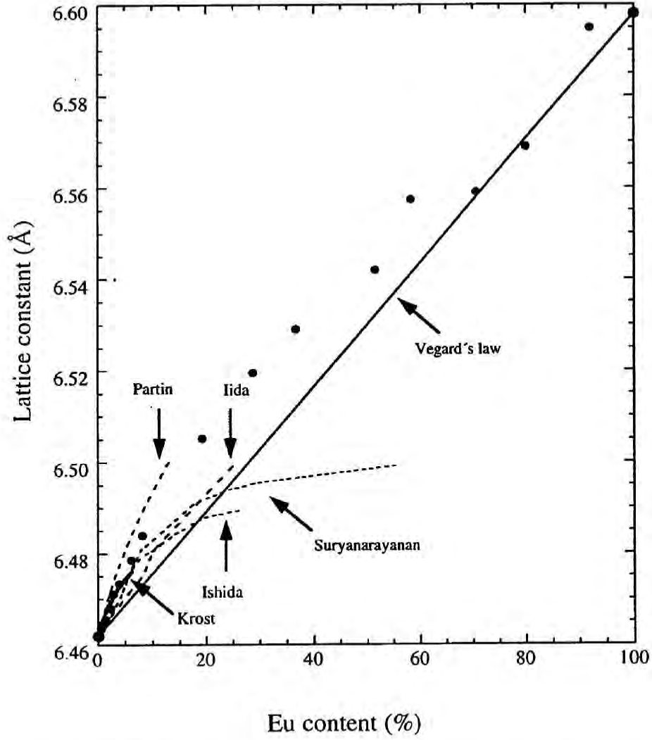
Figure 2-1: Plot for the lattice constant d as a function of Eu content in \text{Pb}_{1-x}\text{Eu}_x\text{Te} alloy [32]. The solid dots indicate the experimental data obtained by Ueta et al. [32]. See Ref. [32] and references therein for the curves obtained by various people.
