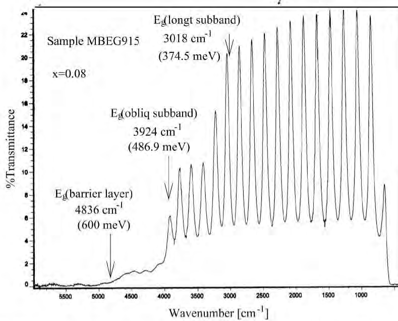
Figure B-10: IR transmission spectrum for a (111) oriented PbTe(20 Å)/Pb 1-x Eu x Te(400 Å) multiple-quantum-well sample (MBEG915). The values of the optical energy band gaps given in the figure are obtained by the Krönig-Penney model using Eqs. B.12 and B.13 to calculate the conduction and valence band offsets at T = 300 K, where the value of x (Eu content) used in the calculation is also given in the figure ( x = 0.08 ).
