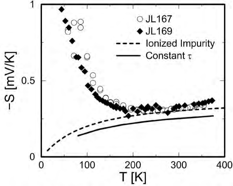
Figure 5-15: Seebeck coefficient as a function of temperature measured for samples JL167 (open circles) and JL169 (filled diamonds), together with theoretical results obtained for n = 4 \times 10^{18} \text{ cm}^{-3} using (1) the constant relaxation time approximation (solid curve) and (2) semiclassical models including ionized impurity scattering as the dominant scattering mechanism (see Chapter 6). The most probable explanation for the rapid increase in the measured Seebeck coefficient |S| is due to the phonon drag effect at the current stage of the investigation (see §5.6.2 and Fig. 5-18 for more discussion).
