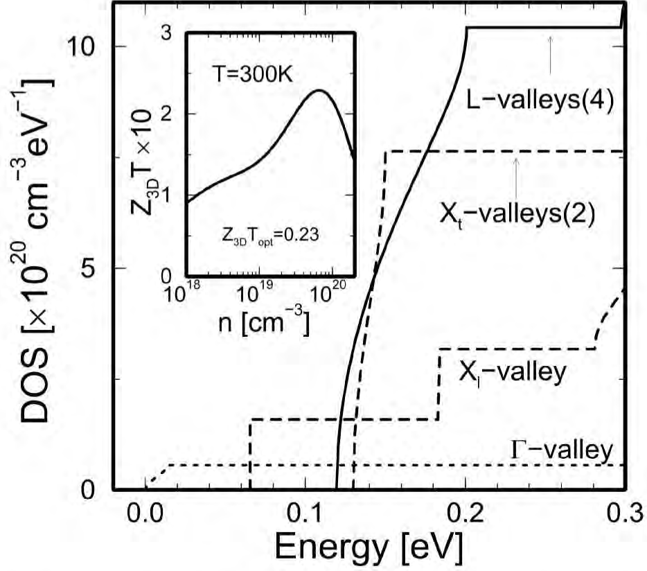
Figure 4-12: Density of states for electrons (DOS) for a (001) oriented GaAs(30 Å)/AlAs(20 Å) superlattice calculated for various subbands derived from \Gamma -, X_l -, X_t - and L -valleys, as indicated in the figure. The number inside the parentheses denotes the number of equivalent valleys that are degenerate in energy. Therefore, the DOS for X_t -valleys shown here, for example, includes contributions from two equivalent X_t -valleys. The inset shows a plot for the calculated Z_{3D}T as a function of carrier concentration n for this superlattice at 300 K. The position of the chemical potential \zeta that gives the optimum value of Z_{3D}T (denoted as Z_{3D}T_{opt} ) is \zeta = 0.154 eV on the main scale.
