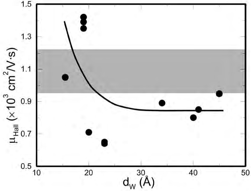
Figure C-1: Hall carrier mobility \mu_{Hall} as a function of the quantum well width d_W for PbTe/Pb 1-x Eu x Te MQWs at 300 K (closed circles). Most of the data are taken from Ref. 2, but a few more recently obtained results are also added. The shaded region indicates the carrier mobilities for similarly grown bulk PbTe for comparison. The solid line is a guide to the eye.
