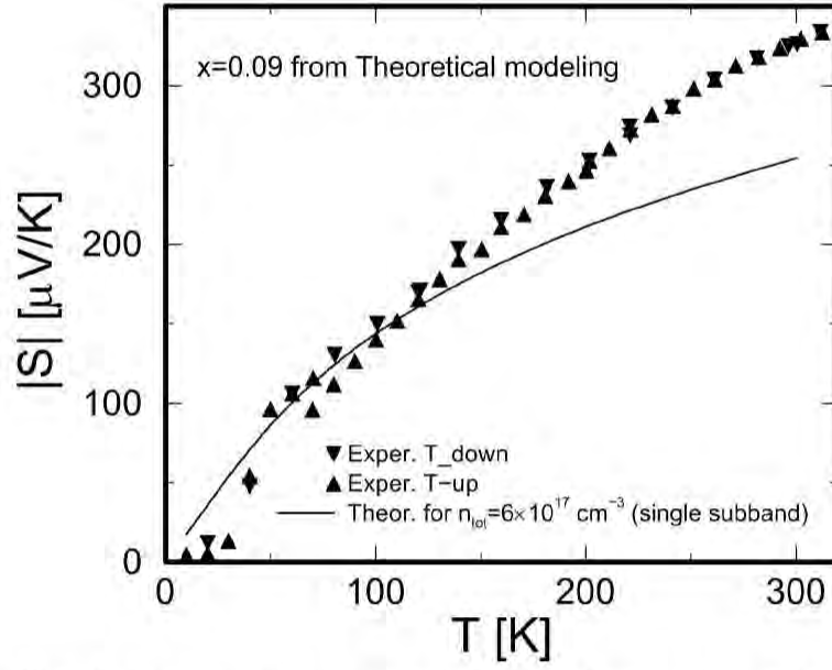
Figure B-17: The Seebeck coefficient as a function of temperature for a (111) oriented \text{PbTe}(20 \text{ \AA})/\text{Pb}_{1-x}\text{Eu}_x\text{Te}(400 \text{ \AA}) multiple-quantum-well sample (MBEG909).
