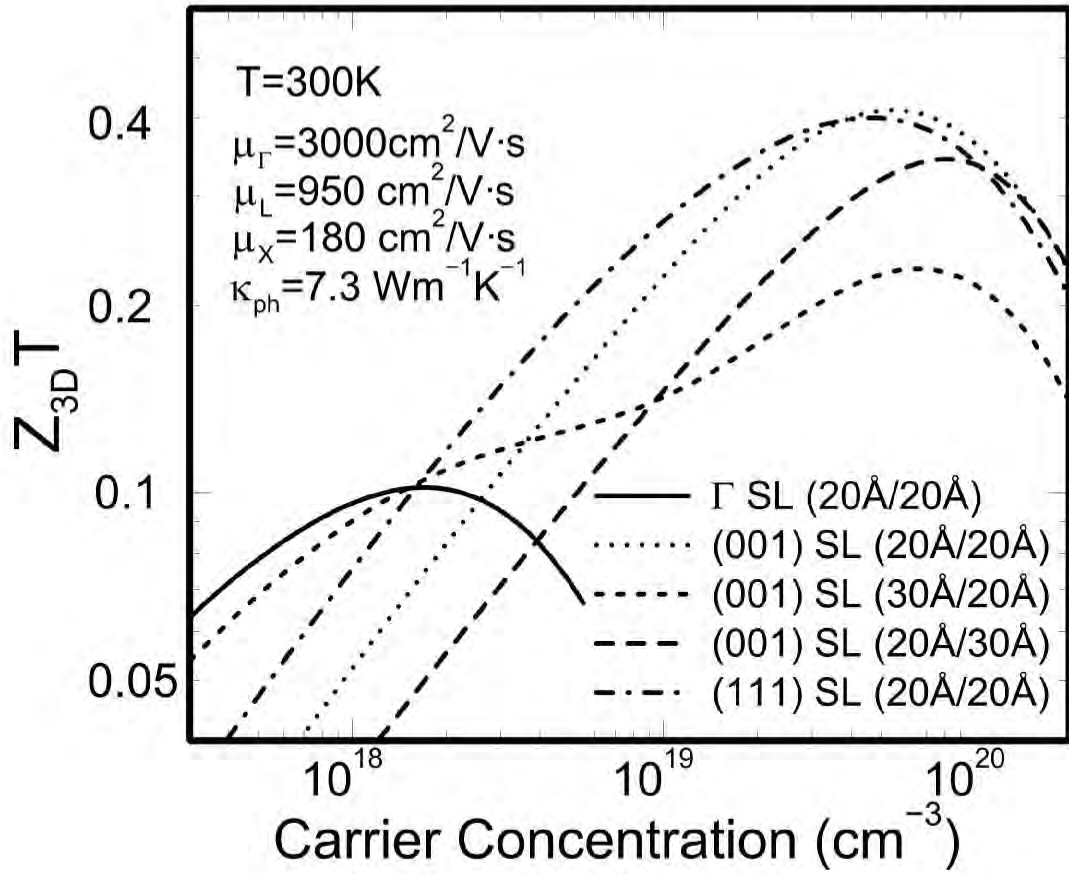
Figure 4-15: Calculated values of Z_{3D}T as a function of carrier concentration for a (001) oriented GaAs(20 Å)/AlAs(20 Å) superlattice (dotted curve), a (001) oriented GaAs(30 Å)/AlAs(20 Å) superlattice (short-dashed curve), a (001) oriented GaAs(20 Å)/AlAs(30 Å) superlattice (long-dashed curve), and a (111) oriented GaAs(20 Å)/AlAs(20 Å) superlattice (long-dash-short-dashed curve). The solid curve denotes Z_{3D}T calculated assuming only carriers in the \Gamma -point subband for a GaAs(20 Å)/AlAs(20 Å) superlattice.
