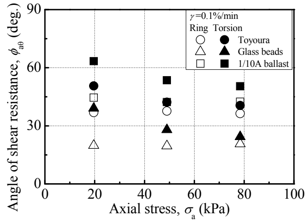
Figure 19. Comparison of angle of shear resistance between multi-ring shear test and hollow cylinder torsional shear test
