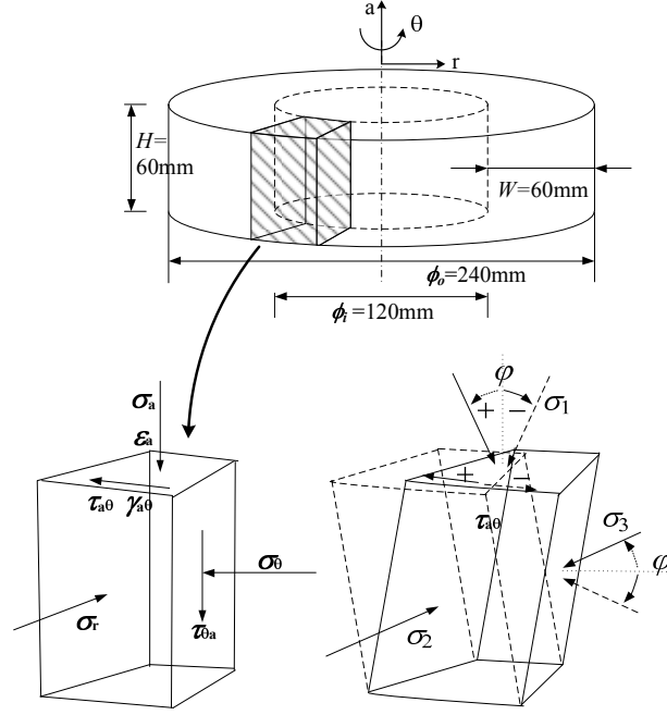
Figure 7. Definition of stress and deformation. \phi , rotational angle of principal stress (major, \sigma_1 ; intermediate, \sigma_2 ; minor, \sigma_3 ); subscript o of \phi refers to the outside diameter and subscript i refers to the inside diameter.
