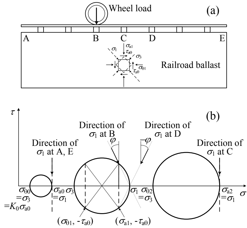
Figure 22. Stresses on a ballast element under a moving-wheel load: (a) stress condition at position C when a loading wheel lies on position B; (b) Mohr's stress circles under a moving-wheel load at various positions.
