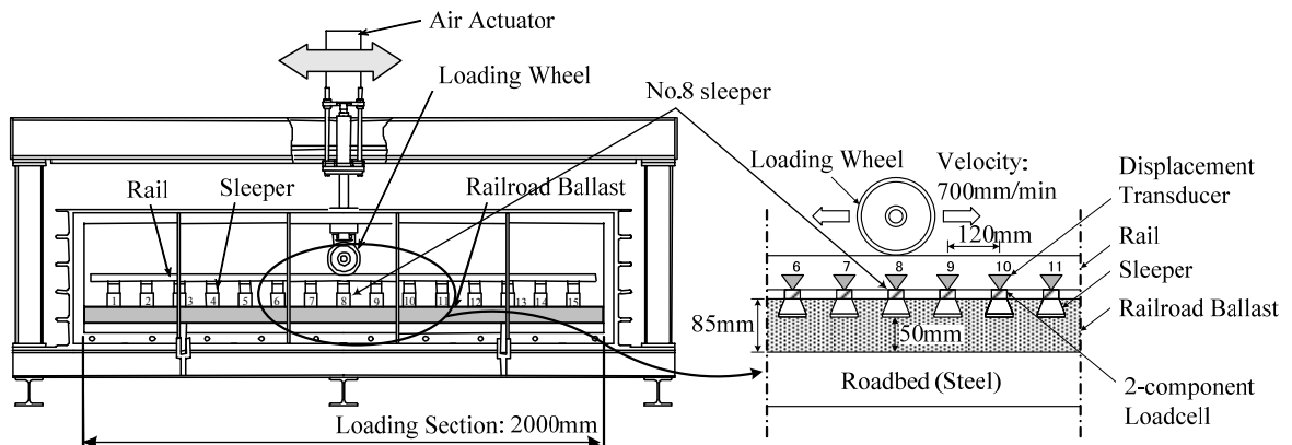
Figure 3. Moving-wheel loading test
