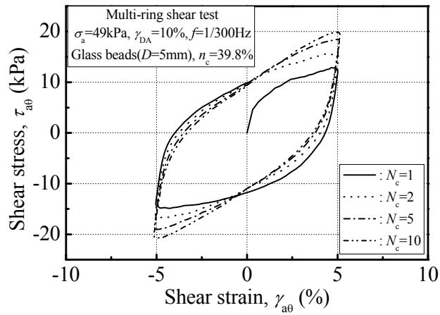
Figure 17. \tau_{a\theta} - \gamma_{a\theta} relationships in cyclic loading multi-ring shear test. n_c , porosity after consolidation; \gamma_{DA} , double amplitude of shear strain.
