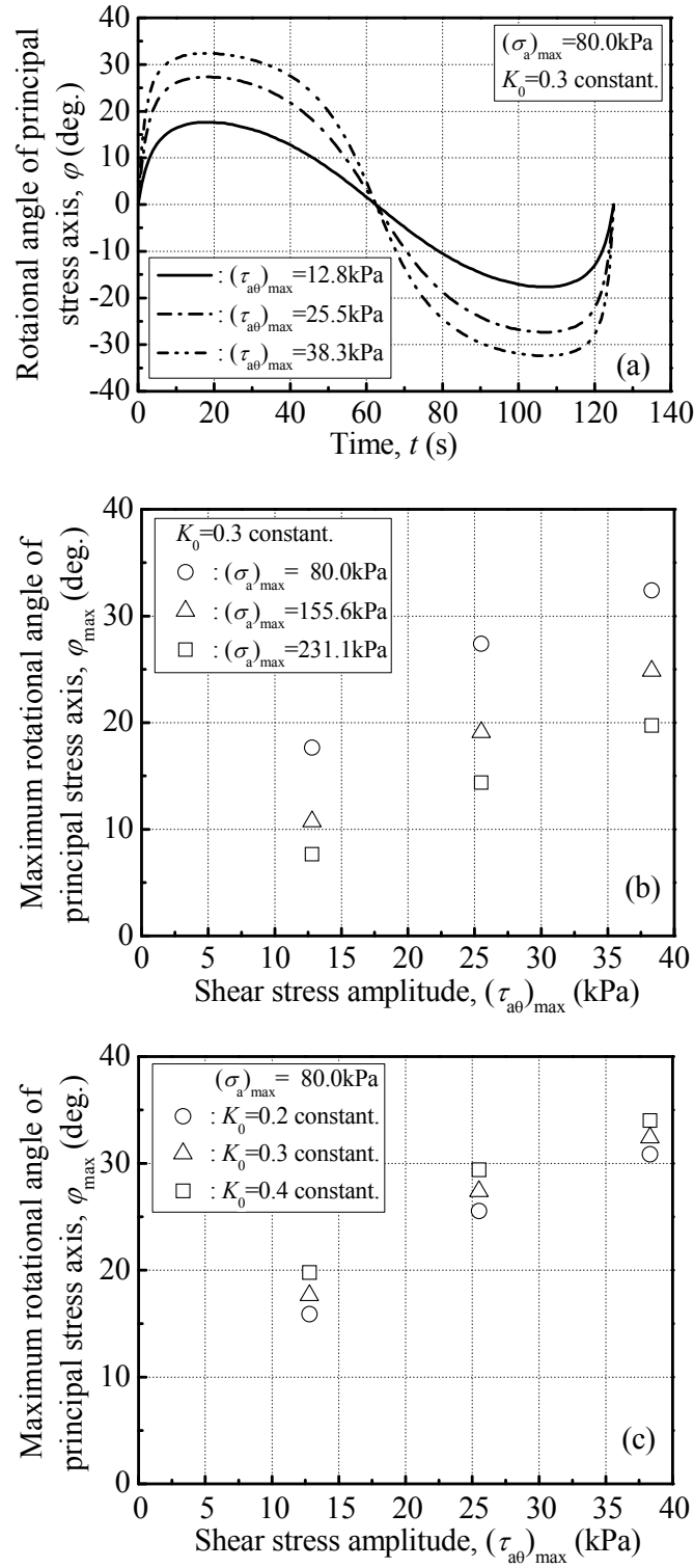
Figure 23. Estimation of principal stress axis rotation in multi-ring shear test using moving-wheel loading mode: (a) rotation of principal stress axis during a loading cycle; (b) effect of loading conditions; (c) effect of coefficient of earth pressure at rest.
