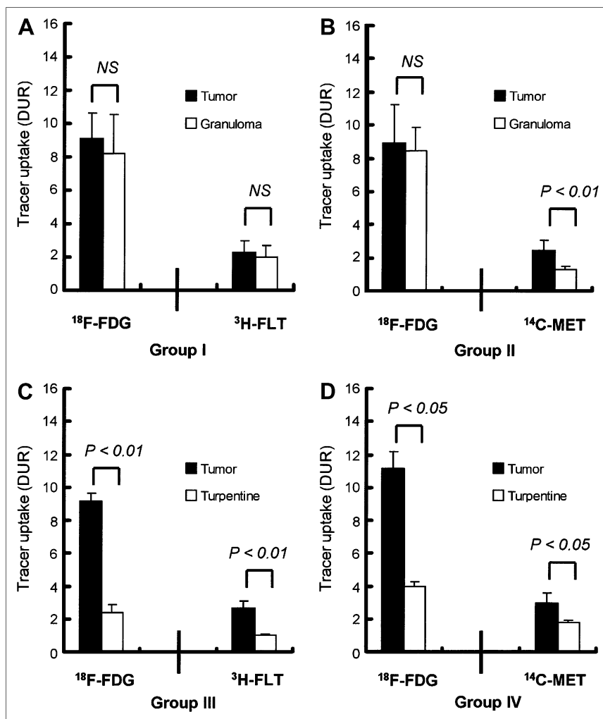
FIGURE 3. ^{18}\text{F} -FDG, ^3\text{H} -FLT, and ^{14}\text{C} -methionine uptake in tumor, granuloma, and turpentine oil-induced inflammation. (A) Group I: ^{18}\text{F} -FDG and ^3\text{H} -FLT uptake in tumor and granuloma. (B) Group II: ^{18}\text{F} -FDG and ^{14}\text{C} -methionine uptake in tumor and granuloma. (C) Group III: ^{18}\text{F} -FDG and ^3\text{H} -FLT uptake in tumor and turpentine oil-induced inflammation. (D) Group IV: ^{18}\text{F} -FDG and ^{14}\text{C} -methionine uptake in turpentine oil-induced inflammation. Values are mean \pm SD. NS = not statistically significant.
