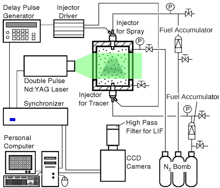
Fig. 2 Schematic of experimental apparatus for LIF-PIV and laser sheet imaging
