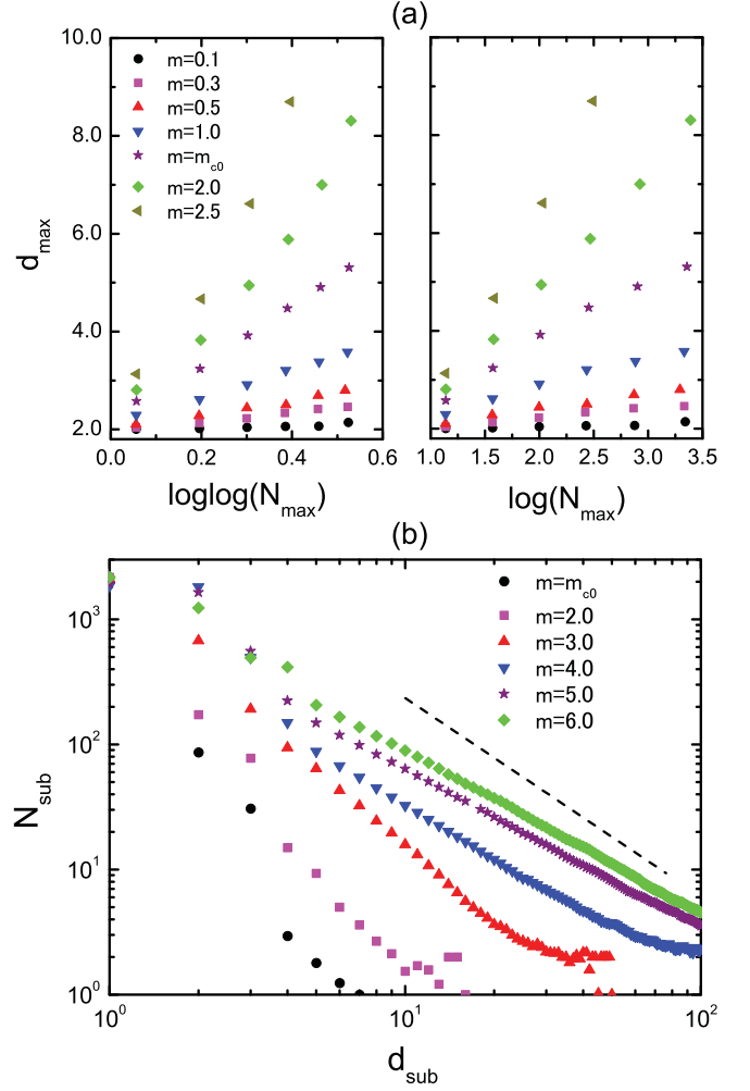
FIG. 7. (Color online) Small-world and fractal properties of Sierpinski geographical networks with \alpha = 2.0 and \langle k \rangle = 4.0 . (a) Upper two panels represent the diameter of the largest connected cluster in Sierpinski geographical networks in the third to eighth generations with one-generation increments as a function of the number of nodes in the cluster. Different symbols indicate results for different values of m . The value of m_{c0} = D/(\alpha - 1) is 1.585. Results are averaged over 10 000 (third generation) to 200 (eighth generation) samples depending on the generation. (b) Lower panel shows the number of subgraphs covering minimally the largest cluster in eighth-generation Sierpinski geographical networks as a function of the diameter of subgraphs. Results are averaged over 200 samples. To achieve the minimum covering, we employed the compact-box-burning algorithm [40]. Dashed line represents the slope of the fractal dimension D = \ln 3 / \ln 2 .
