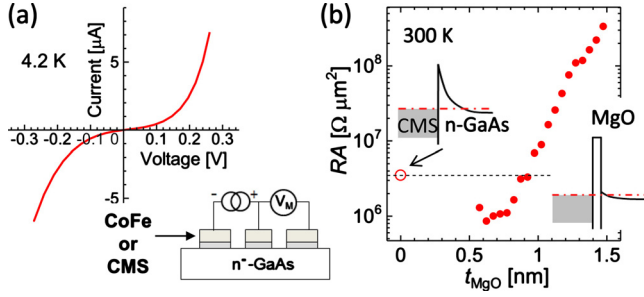
FIG. 2. (Color online) (a) Current-voltage characteristics of a \text{Co}_2\text{MnSi} (CMS)/n-GaAs Schottky tunnel junction measured at 4.2 K. The inset shows a circuit configuration for three-terminal geometry. (b) RA products of CMS/MgO/n-GaAs single junctions at RT as a function of MgO thickness. The inset shows schematic band diagrams of CMS/n-GaAs junctions with and without a MgO barrier.
