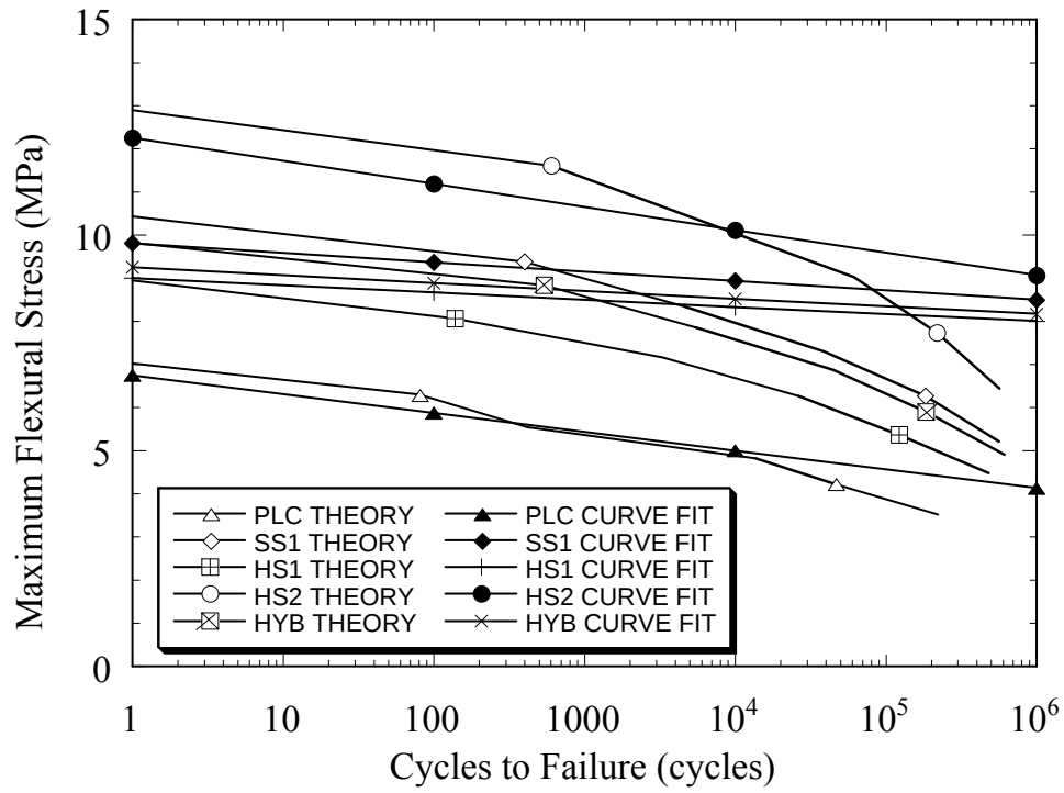
Figure 17 Theoretical S-N diagram and curve fit to experimental data 25 of plain concrete and four FRCs.
