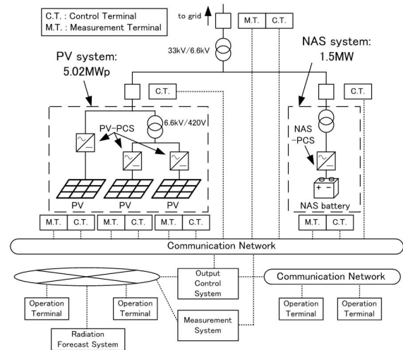
Figure 1 Outline of Wakkanai Power Station.
