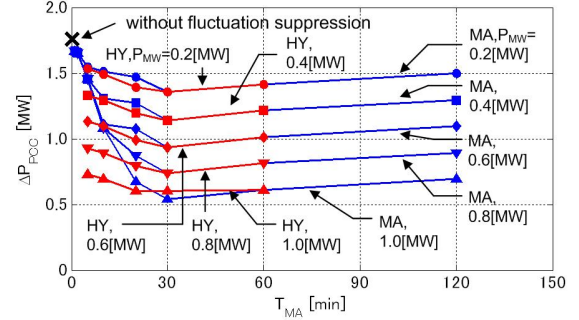
Figure 5 Relation between T_{MA} , P_{MW} , and \Delta P_{PCC} .
