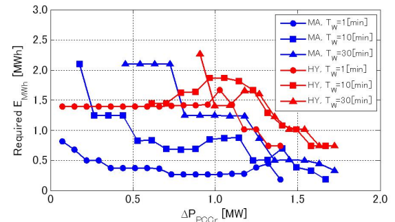
Figure 7 Required E_{MWh} to satisfy \Delta P_{PCCR} .
