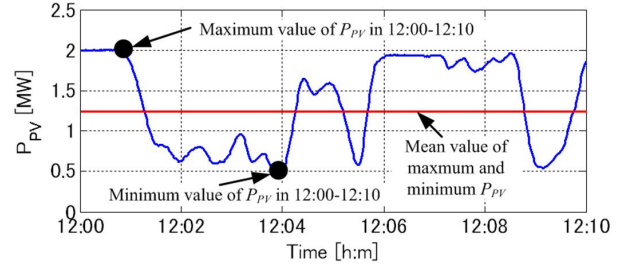
Figure 4 Mean Value of Maximum and Minimum P_{PV} .
