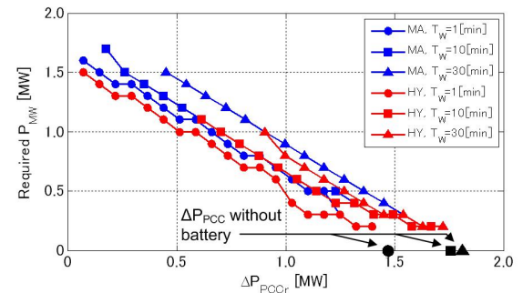
Figure 6 Required P_{MW} to satisfy \Delta P_{PCCR} .
