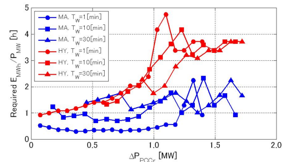
Figure 8 Required E_{MWh}/P_{MW} to satisfy \Delta P_{PCCR} .
