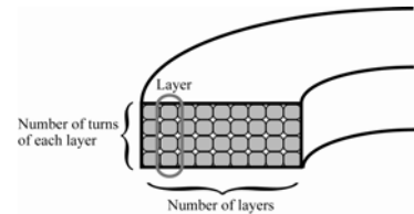
Fig. 3. Schematic view of the layer and the turn of each layer of the element coil. The numbers of layers and turns of each layer are the design variables.
