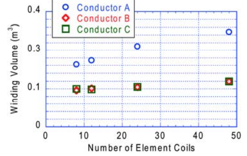
Fig. 7. The winding volume of the optimized DCL magnet using the Conductors A, B and C.
