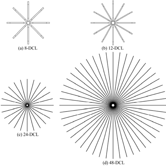
Fig. 4. Optimization configurations of the toroidal superconducting magnet for DCL. The operating temperature is 77 K. The figures show the actual proportion of coils.
