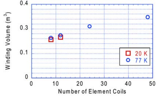
Fig. 5. The relation between the number of element coils and the winding volume at the operating temperatures 20 K and 77 K.
