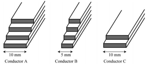
Fig. 6. The conductors used in optimal design of DCL magnet. The Conductor A consists of 4 sheets of YBCO with a width of 10 mm, the Conductor B 4 sheets of YBCO with a width of 5 mm, and Conductor C 2 sheets of YBCO with a width of 10 mm.
