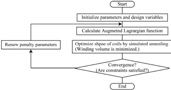
Fig. 1. Flowchart of the optimization algorithm combining the simulated annealing and the Augmented Lagrange multiplier method.
