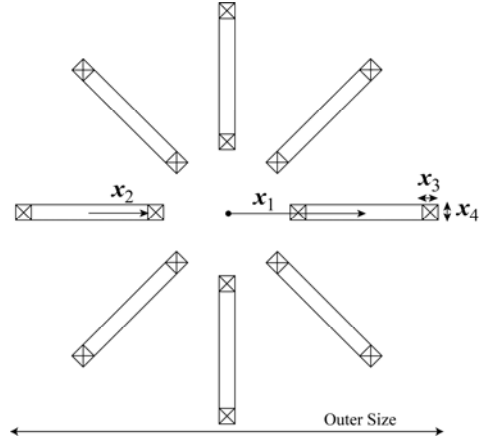
Fig. 2. Design model of toroidal magnets and 4 design variables for optimal design, x_1 , x_2 , x_3 , and x_4 are the distance between the center of toroid and the center of an element coil, the inner radius of each element coil and the thickness and length of each element coil, respectively.
