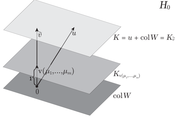
Figure 3: K_{v(\mu_1, \dots, \mu_m)} .
