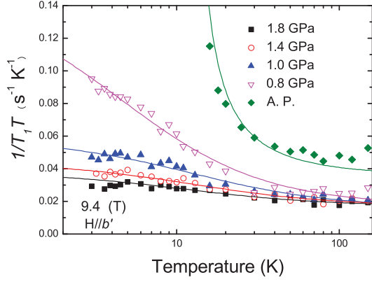
FIG. 5. (Color online) Temperature dependence of (T_1T)^{-1} at ambient and other pressures.
