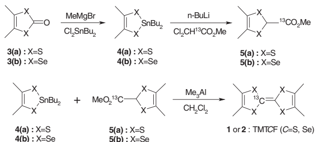
FIG. 2. Synthetic route to prepare single-site ^{13}\text{C} -enriched TMTCF.
