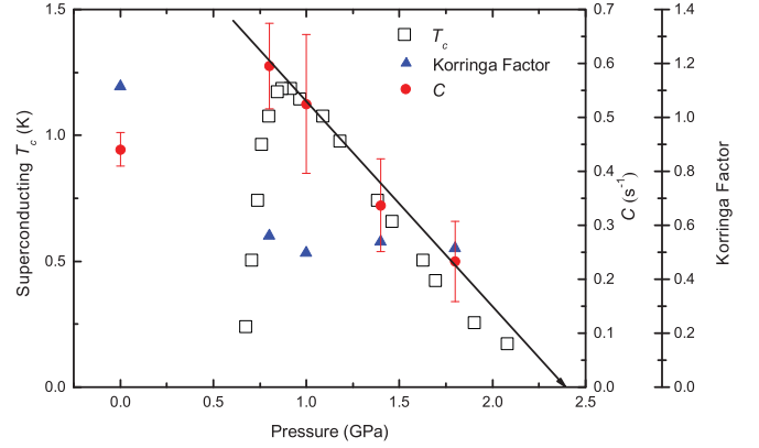
FIG. 7. (Color online) Pressure dependence of T_c , C , and the Korringa factor \mathcal{K}^5 .
