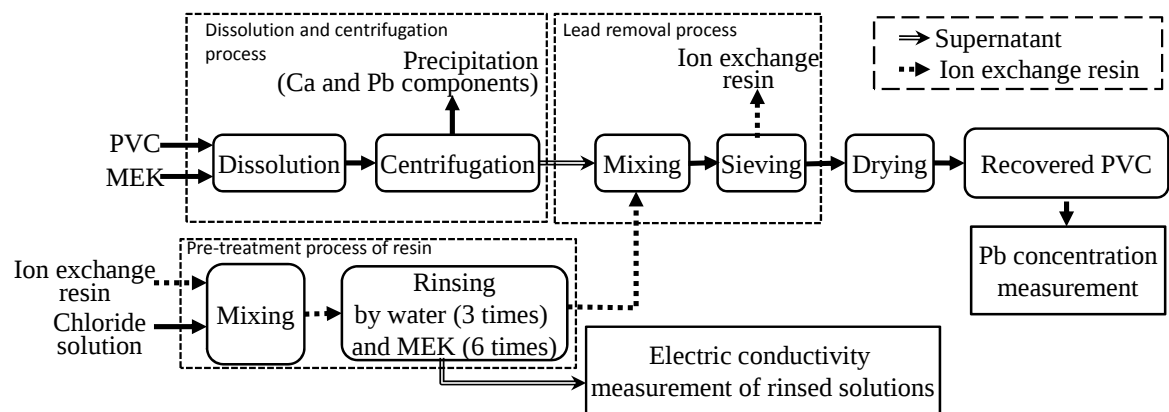
Fig. 1 Flowchart of the lead removal treatment process.
