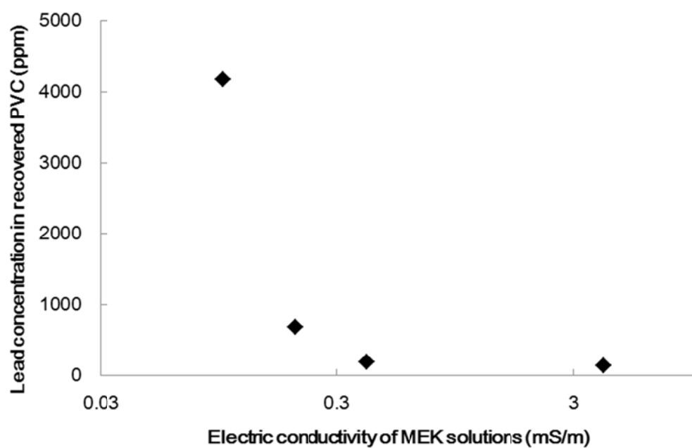
Fig. 6 Relationship between the lead concentration in the recovered PVC and the electric conductivity of the HCl containing MEK solutions used in the dissolution process (the amount of added hydrochloric acid solution is 1 mass% for MEK).
