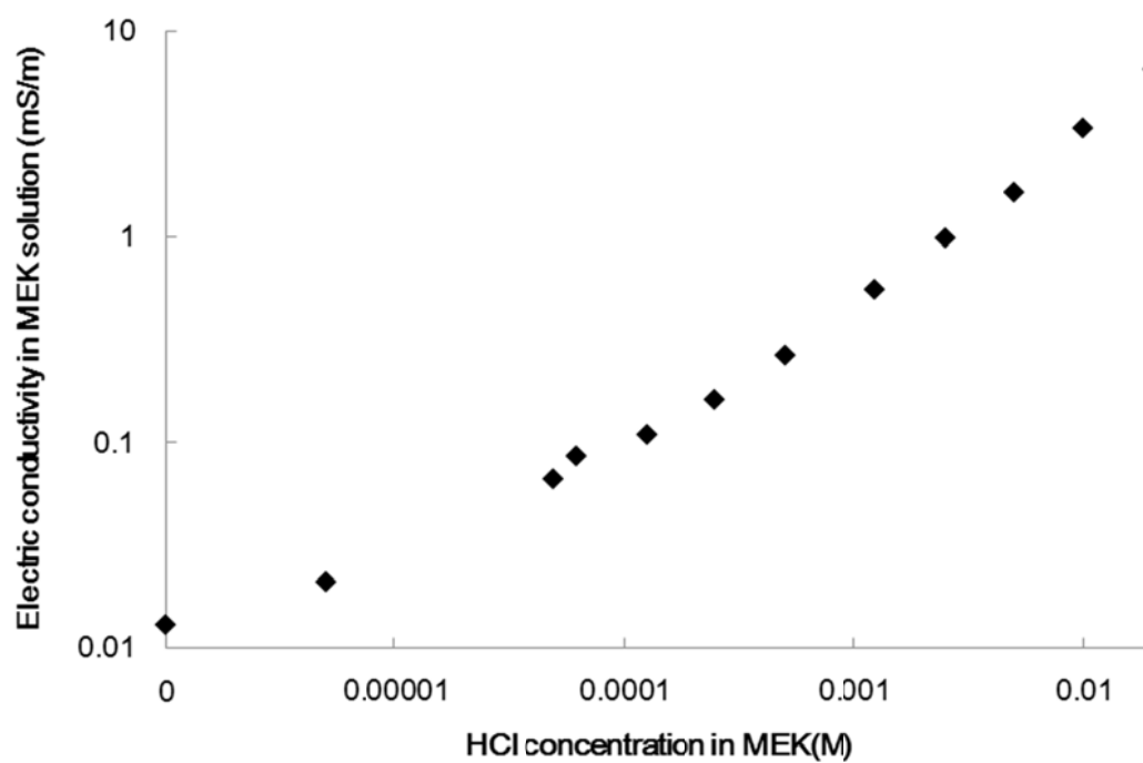
Fig. 5 The electric conductivity of the HCl containing MEK solutions (the amount of added hydrochloric acid solution is 1 mass% for MEK and the value of '0 M' shows the conductivity of the MEK containing 1 mass% of H 2 O).
