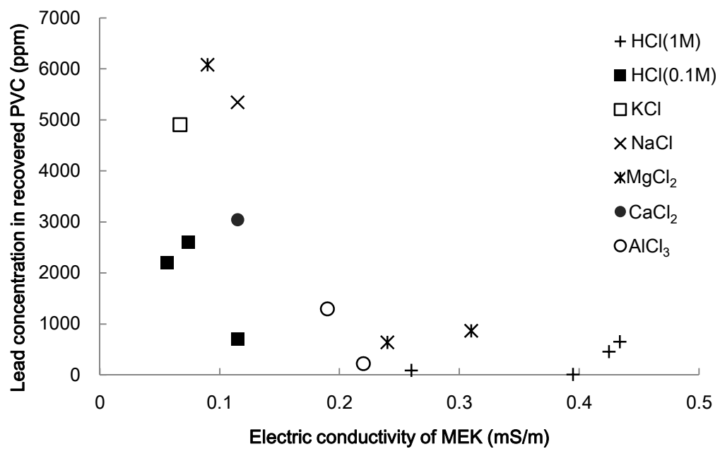
Fig. 4 Relationship between the lead concentration in the recovered PVC and the electric conductivity of the MEK used in the last rinsing of the ion exchange resin.
