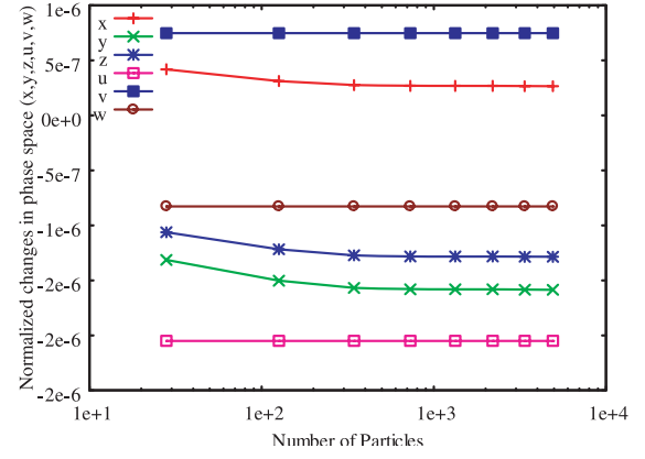
Fig. 3 Convergence of the ALG with the number of particles N : Changes in position and in velocity of a test particle.
