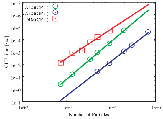
Fig. 5 CPU time vs the number of particles N with fitting lines, \tau_{ALG}^{CPU} \sim 5.56 \times 10^{-9} N^{3.02} for the ALG on a CPU in green, and \tau_{DIM}^{CPU} \sim 3.06 \times 10^{-5} N^{2.34} for the DIM on the CPU in red. Also depicted are CPU times for ALG-GPU calculations with a fitting line \tau_{ALG}^{GPU} \sim 1.88 \times 10^{-9} N^{2.75} in blue.
