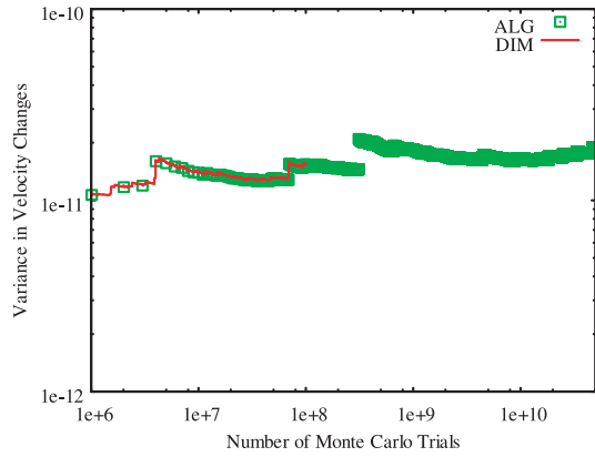
Fig. 4 Normalized variance of velocity changes for N = 28 by using the ALG with N_{MC} = 5 \times 10^{10} , while up to N_{MC} = 10^8 for the DIM.
