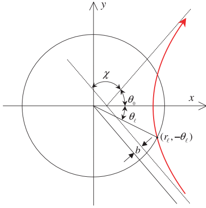
Fig. 1 Unperturbed relative trajectory r = r(\theta) in an orbital plane for the repulsive force. The scattering center is at the origin. An impact parameter is b = b_0 \tan \theta_0 .
