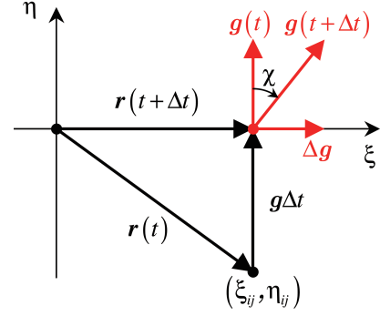
Fig. 2 Coordinate transform from the (x, y, z) to (\xi, \eta) , in such a way that the third axis, say \zeta , is set parallel to the angular momentum \mathbf{L} = \mathbf{r} \times \mu \mathbf{g} = L \mathbf{e}_\zeta , and \mathbf{g} = g \mathbf{e}_\eta . In this coordinate system, the scattering angle \chi , i.e., the impact parameter b and the time of the interaction \Delta t are approximately given by \xi and \eta , respectively. The relative velocity at time t and t + \Delta t , are \mathbf{g}(t) , and \mathbf{g}(t + \Delta t) = \mathbf{g}(t) + \Delta \mathbf{g} , respectively.
