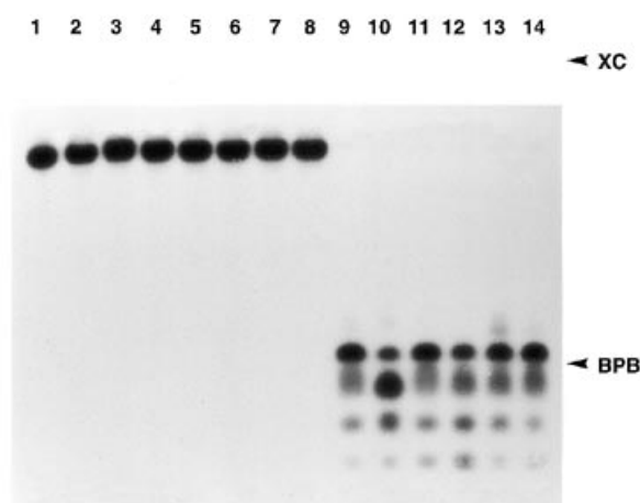
Figure 5. Polyacrylamide gel electrophoresis of 5'- 32 P-labeled RNA hydrolyzed by E. coli RNase H (6.0 U). ODN-RNA duplexes were incubated with E. coli RNase H for 20 min at 30°C: lane 1, RNA; lane 2, RNA + enzyme; lane 3, RNA + gap 1; lane 4, RNA + gap 2; lane 5, RNA + gap 3; lane 6, RNA + gap 4; lane 7, RNA + gap 5; lane 8, RNA + control; lane 9, RNA + gap 1 + enzyme; lane 10, RNA + gap 2 + enzyme; lane 11, RNA + gap 3 + enzyme; lane 12, RNA + gap 4 + enzyme; lane 13, RNA + gap 5 + enzyme; lane 14, RNA + control + enzyme. Experimental conditions are described under Materials and Methods.
