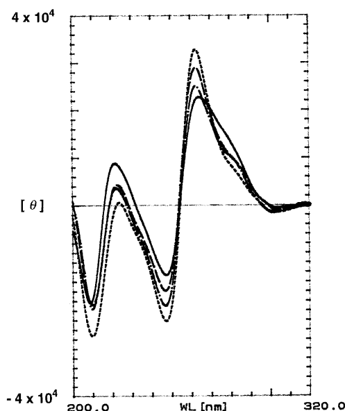
Figure 2. CD spectra of ODN-RNA duplexes at 10°C in 0.01 M NaCl, 0.01 M sodium cacodylate (pH 7.0). (—) control-RNA; (---) gap 1-RNA; (- - -) gap 3-RNA; (- · -) gap 5-RNA.
