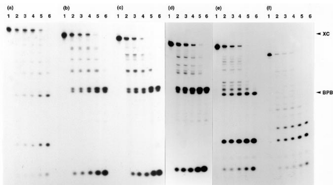
Figure 3. Polyacrylamide gel electrophoresis of 5'- 32 P-labeled ODNs hydrolyzed by nuclease S1: (a) gap 1; (b) gap 2; (c) gap 3; (d) gap 4; (e) gap 5; (f) control. ODNs were incubated with nuclease S1 for 0 min (lane 1), 10 min (lane 2), 20 min (lane 3), 30 min (lane 4), 60 min (lane 5), and 120 min (lane 6). Experimental conditions are described under Materials and Methods.
