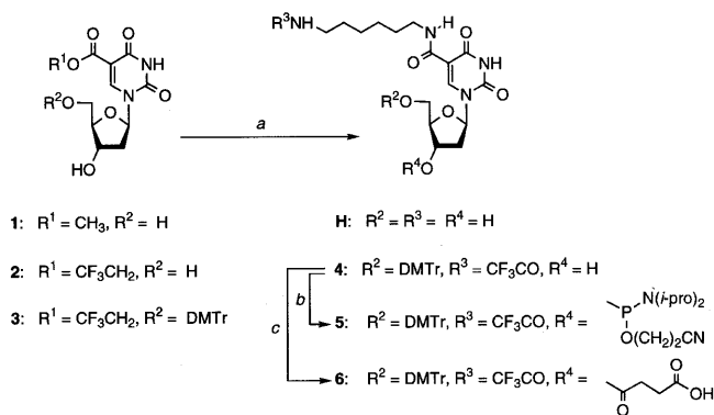
Scheme 1. (a) (1) NH 2 (CH 2 ) 6 NH 2 , pyridine, room temperature, (2) CF 3 COOEt, Et 3 N, DMF, room temperature; (b) 2-cyanoethyl N,N -diisopropylphosphoramidochloride, N,N -diisopropylethylamine, CH 2 Cl 2 , room temperature; (c) succinic anhydride, DMAP, pyridine, room temperature.
