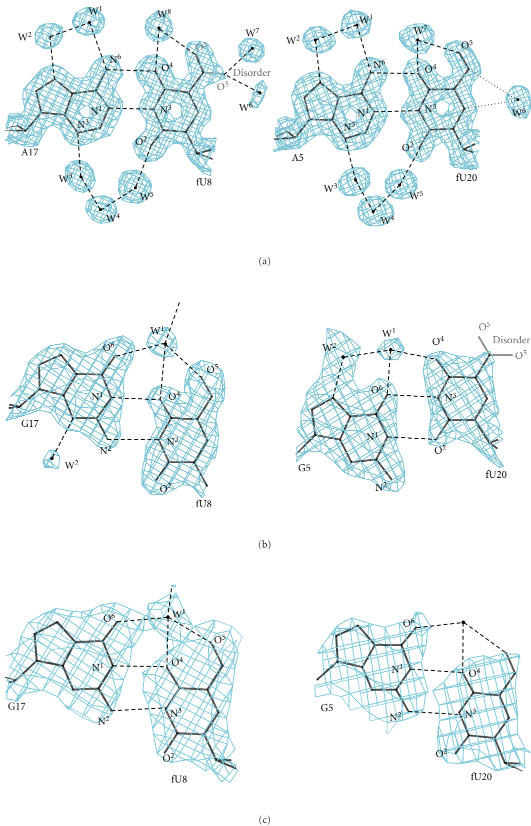
FIGURE 1: The final 2|F_o| - |F_c| maps around the fU residues in the fUA 2 (a), the fUG 2 (b), and the fUG 3 (c) crystals. The maps are contoured at 1\sigma level by the program DINO [18]. Those of the fUG 1 crystal are omitted due to similarity to (c). Values indicate possible hydrogen bond distances. Characters N, O, and W indicate nitrogen, oxygen, and water oxygen atoms, respectively.
