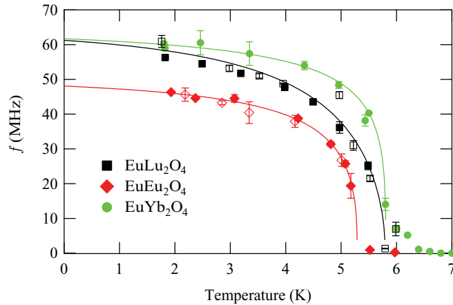
FIG. 3. (Color online) Temperature dependence of the muon-spin precession frequency ( f \equiv \omega_{AF}/2\pi ) of L = \text{Eu, Lu, Yb} . Filled symbols were measured in ZF, hollow symbols were measured in wTF. Lines indicate the T dependence of the BCS gap energy.
