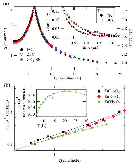
FIG. 5. (Color online) \text{EuYb}_2\text{O}_4 : (a) inset shows the raw ZF asymmetries taken at 7 and 30 K. Main panel depicts the \text{EuYb}_2\text{O}_4 temperature dependence of the zero-field (ZFC) and field-cooled (FC) susceptibility \chi = M/H (left axis) and the muon T_1^{-1} relaxation rate (right axis). (b) Inset shows the temperature dependence of 1/(T_1 T \chi) . Main panel displays (T_1 T)^{-1} versus \chi for \text{EuLu}_2\text{O}_4 , \text{EuEu}_2\text{O}_4 , and \text{EuYb}_2\text{O}_4 . The solid lines in the figures display the fit.
