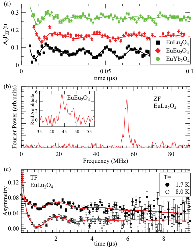
FIG. 2. (Color online) (a) The raw ZF data of EuLu 2 O 4 , taken at T = 1.8 K, solid lines demonstrate the fit. The data of L = \text{Eu} , Yb are shifted by +0.1 and +0.2 for clarity. (b) The ZF FT of EuLu 2 O 4 , taken at T = 1.8 K; inset shows the real part of the FT of EuEu 2 O 4 at T = 1.8 K. (c) Measurements in wTF taken at 1.7 and 8.0 K; the asymmetry of the 1.7 K data is shifted by 0.05 for clarity. The solid lines indicate the fits.
