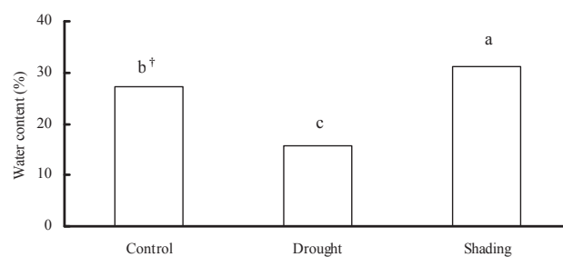
Fig. 1. Soil water content in each treatment at 45 d after emergence. † Different letters indicate differences among treatments based on the LSD test ( P \leq 0.05 ).
