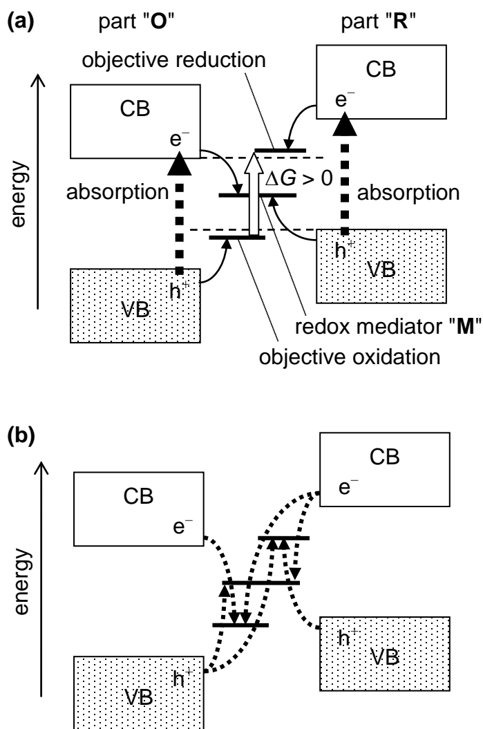
Fig. Z (a) A Z-scheme reaction combining two semiconductor photocatalytic reaction parts ("R" and "O") with a redox mediator "M". (b) Undesired possible e^- and h^+ transfer processes in a Z-scheme inducing "short circuiting" of a target reaction.
