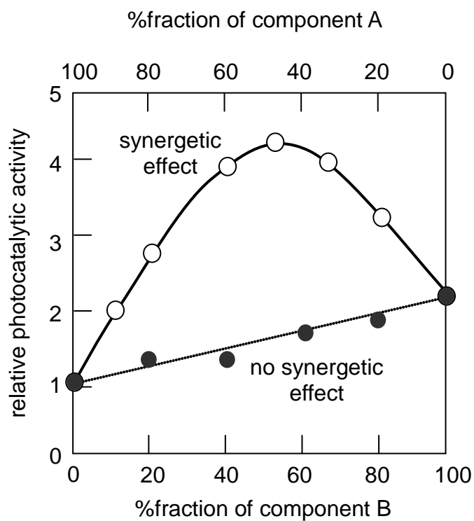
Fig. S Hypothetical representation of relative photocatalytic activities of mixtures of components A and B. A synergetic effect can be suggested at least when a mixture shows better photocatalytic activity compared with those of pure components A and B.
