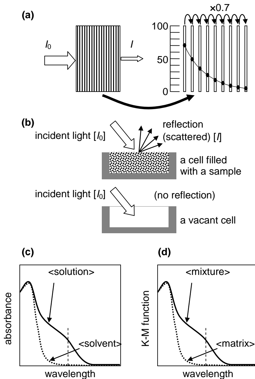
Fig. K (a) Logarithmic decrease in light intensity by absorption at constant (e.g. 30%) absorption at each thin layer. (b) Extinction (absorption and scattering) measurement for solid samples requires a standard sample which reflects incident light. Examples of measurements of (c) absorbance and (d) Kubelka-Munk function (K-M function) for homogeneous liquid and solid powder samples, respectively. Components in (c) solvent and (d) powder matrix give shoulder peaks and their absorbance and K-M function are proportional to their concentration, but not extent of photoabsorption in (c) solvent and (d) matrix, respectively.
