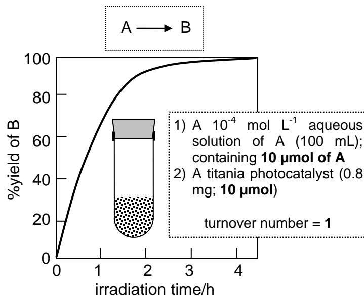
Fig. Y An example of calculation of turnover number in photocatalytic conversion of A into B. %Yield can not show turnover of the photocatalyst.
