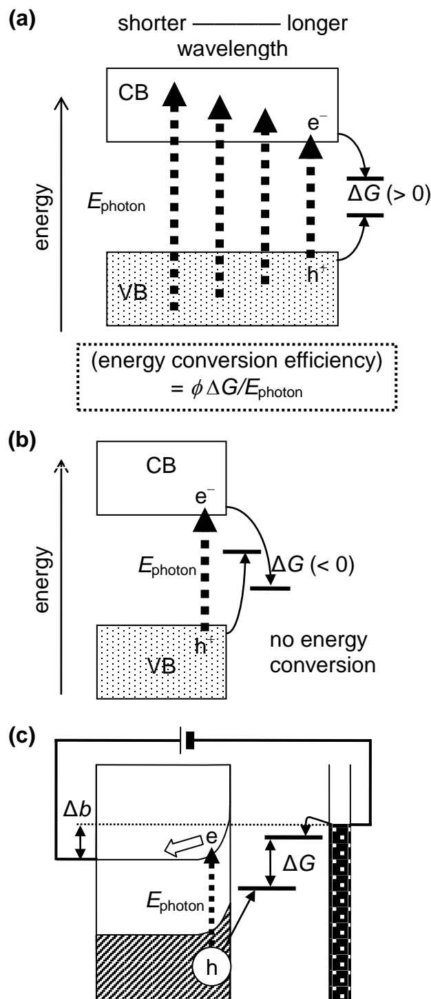
Fig. E (a) Light-to-chemical energy conversion efficiency of photocatalytic reaction calculated as an integral of a product of apparent quantum efficiency ( \phi ) and Gibbs energy change (storage) divided by photon energy ( E_{\text{photon}} ) as a function of wavelength. (b) In the case where Gibbs energy change is negative, energy conversion efficiency can not be defined, or is defined to be zero. (c) Electrochemically biased ( \Delta b ) photoelectrochemical cell consisting of an n-type semiconductor and metal counter electrodes.
