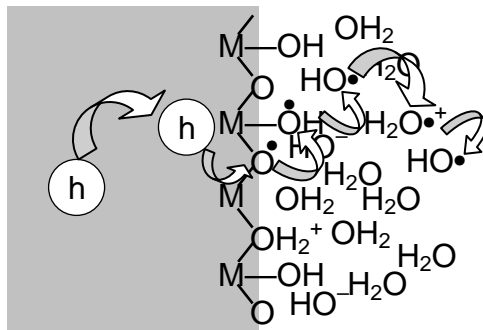
Fig. H Transfer of positive holes from the bulk of a photocatalyst through the interface to aqueous solution phase. Surface-adsorbed and free (hydrated) hydroxyl radicals and their derivatives can be a possible form of positive holes.
