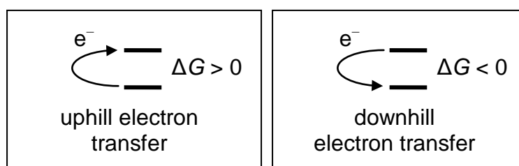
Fig. T Gibbs-energy change in photocatalytic reactions by a photocatalyst of a molecule or a highly dispersed compound.
