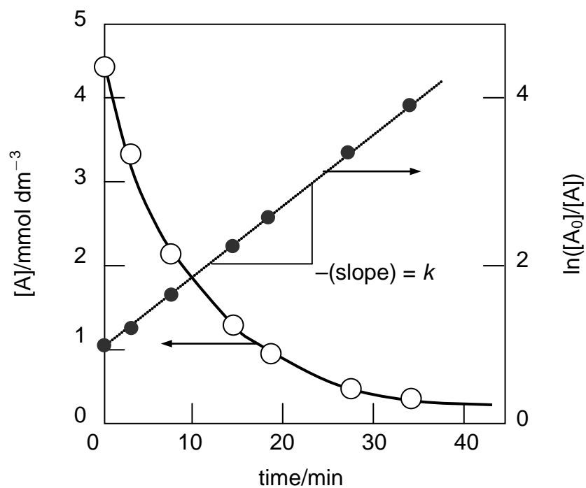
Fig. F First-order kinetic analysis for a reaction consuming a substrate A. Plot of logarithm of relative consumption (in the present plot, ratio of initial concentration of substrate A and concentration of A at a given time).
