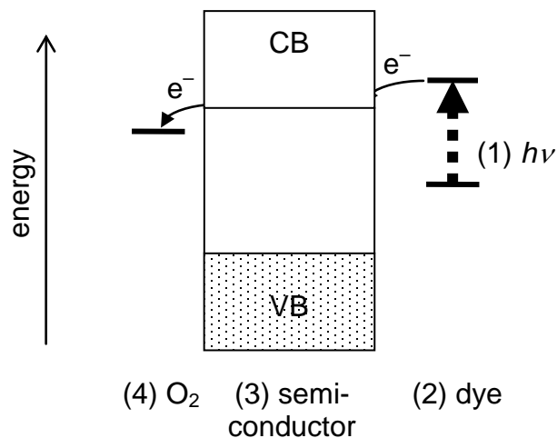
Fig. V Possible mechanism of "dye-sensitized" photoinduced oxidative decomposition of dye in the presence of oxygen. Components (1)–(4) are necessary conditions for "dye-sensitized reaction" and they are also necessary conditions for ordinary photocatalytic reaction.
