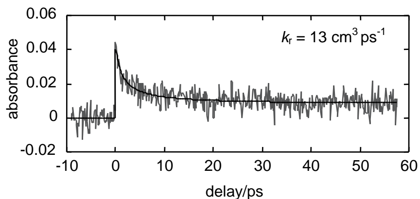
Fig. M An example of picosecond-time-region decay of photoabsorption (620 nm) of trapped electrons in Degussa (Evonik) P25 particles after excitation by a ca. 100-fs pump pulse (310 nm). The curve was analyzed by a second-order rate law ( eq. M ) with a baseline component ( BL ), and a second-order rate constant ( k_r ) was obtained to be 13 \text{ cm}^3 \text{ ps}^{-1} .
