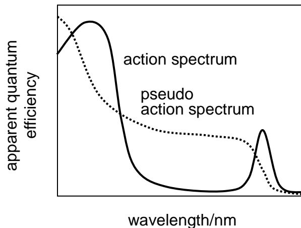
Fig. W Examples of action (solid line) and pseudo action (dotted line) spectra for photoinduced reaction by an ordinary semiconductor photocatalyst (shorter wavelength) and an organic dye (longer wavelength peak). A pseudo action spectrum taken by cut-off filters corresponds to integration of the "true" action spectrum from the longer-wavelength side.
