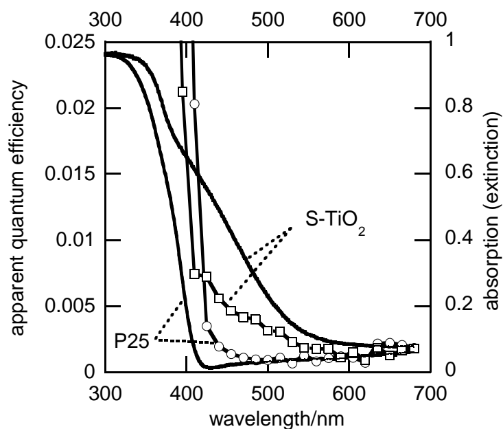
Fig. D Diffuse reflectance (photoabsorption) and action spectra for acetic acid decomposition in aerated aqueous solutions of sulfur-doped titania (S-TiO 2 ) and Degussa (Evonik) P25.
