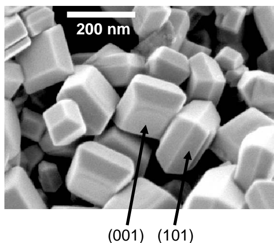
Fig. N A representative SEM image of decahedral anatase-titania particles prepared by controlled gas-phase reaction of titanium(IV) chloride and oxygen at 1473 K. Most particles expose two square (001) facets and eight trapezoidal (101) facets.
