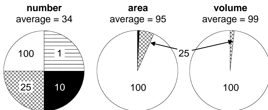
Fig. P Example of fractions of four kinds of particles (25% each in number) of size 1, 10, 25 and 100 nm in number, area and volume (weight). Figures in circle graphs show the particle size. Average size of particles is calculated on the basis of fractions.
