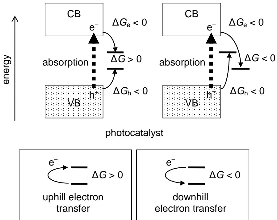
Fig. G Gibbs-energy change in photocatalytic reactions.
