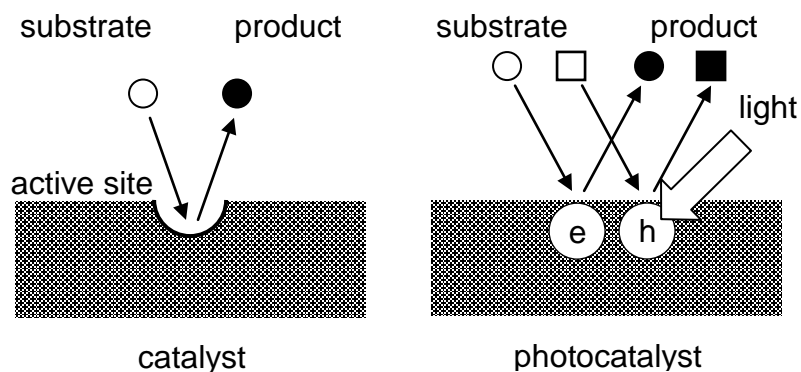
Fig. A Difference in concepts of catalytic and photocatalytic reactions: A catalyst contains active sites of which a substrate is converted into a product, while no active sites are present on a photocatalyst.
