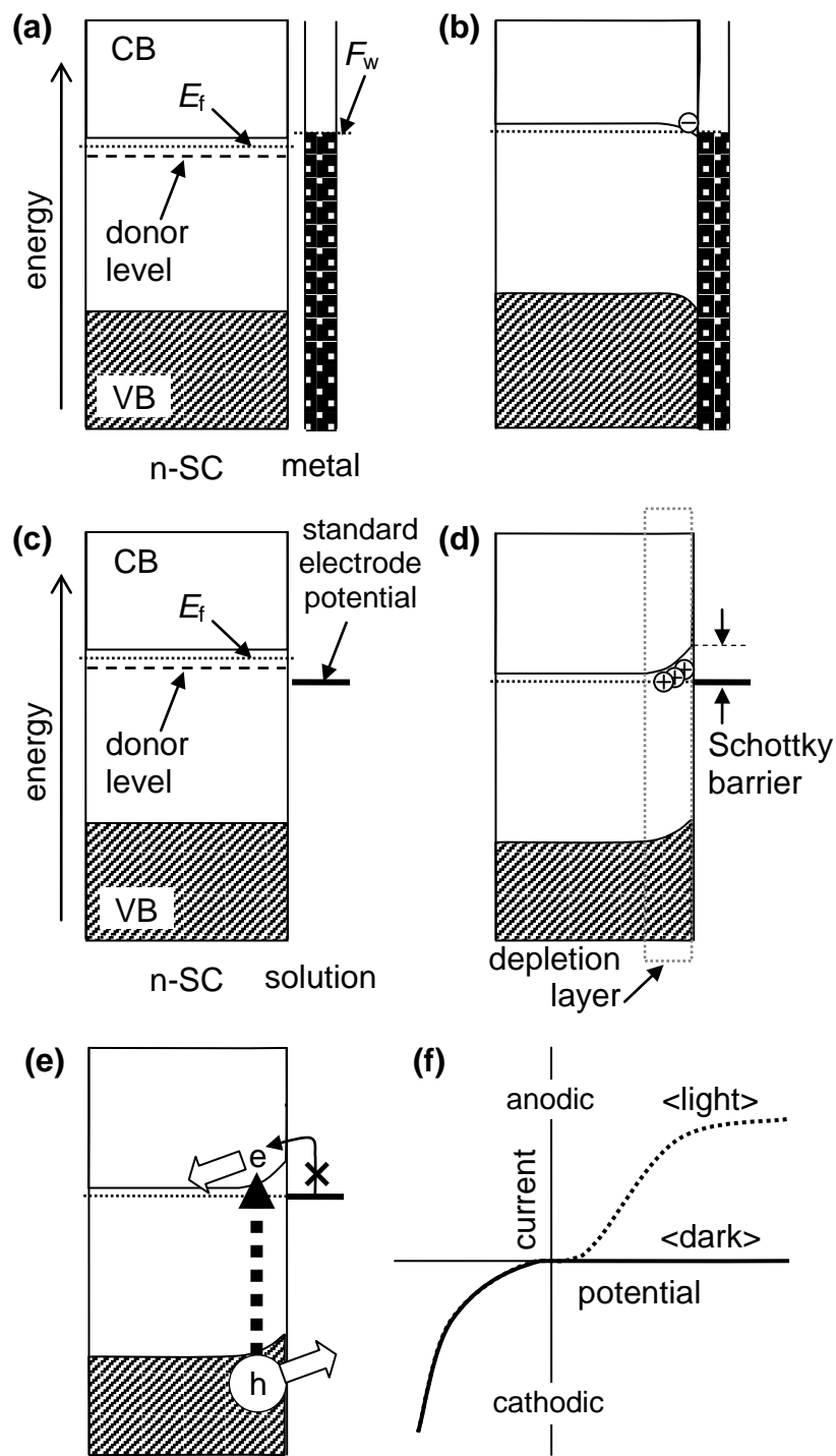
Fig. J (a) n-SC and metal with work function ( F_w ) and (b) ohmic contact between them. (c) N-type semiconductor (n-SC) and solution and (d) Schottky junction with a depletion layer where electrons in donor levels flew out to the solution to lower the Fermi level ( E_F ). (e) n-SC–electrolyte interface under photoirradiation and (f) ideal potential–current plots in the dark and under photoirradiation.
