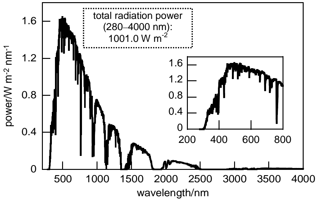
Fig. U A solar spectrum drawn on the basis of data of solar radiation at the ground surface in the temperate zone (AM1.5) reported by the American Society for Testing and Materials (ASTM, http://www.astm.org/ ASTM). An inserted spectrum is a magnified drawing for a part of ultraviolet and visible light.
