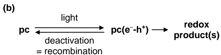
Fig. R (a) Model interpreting a rate-determining step in a 4-step series reaction. Step 3 with largest activation energy determines the overall rate. (b) Simplified scheme of photocatalytic reaction with a photocatalyst "pc". It is clear that this process is not a series reaction since a "deactivation step" is included.
