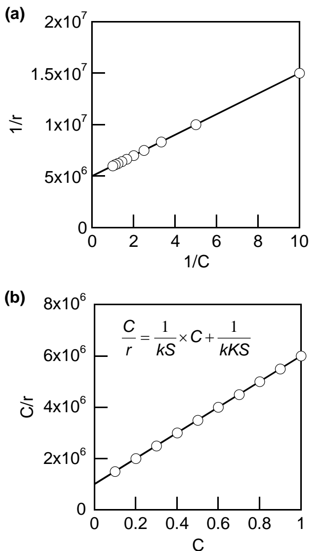
Fig. L Simulation of linearized plots for kinetics governed by surface concentration of substrates adsorbed on the photocatalyst surface in a Langmuirian fashion, where r , C , k , K and S are rate of reaction ( \text{mol s}^{-1} ), concentration of a substrate ( \text{mol L}^{-1} ), rate constant ( 10^{-4} \text{ s}^{-1} ), adsorption equilibrium constant ( 5 \text{ L mol}^{-1} ) and saturated amount of adsorption ( 2 \times 10^{-3} \text{ mol} ).
