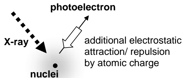
Fig. X Chemical shift in X-ray photoelectron spectra appears by interaction or repulsion by possible positive charge when photoelectrons are escaping from atomic nuclei, while no effect of neighboring atoms is expected.
