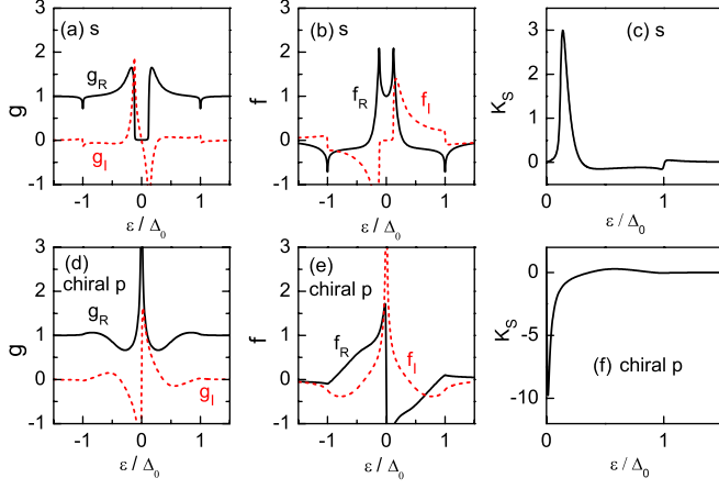
FIG. 2 (color online). The retarded Green functions at the surface of the normal metal for the s wave (a),(b) and the chiral p -wave symmetry (d),(e). The solid and broken lines represents the real and imaginary part of the Green function, respectively. In (c) and (f), K_s is the spectral pair density and corresponds to the kernel of the imaginary part of complex conductivity at \omega \rightarrow 0^+ .
