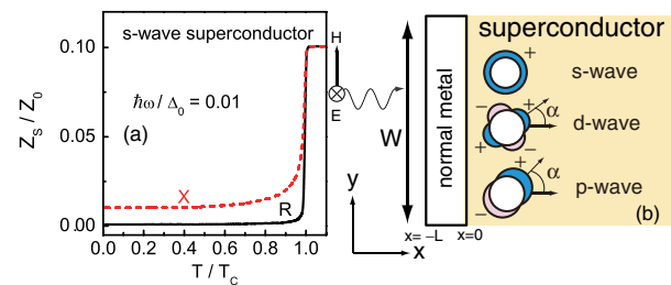
FIG. 1 (color online). (a) Typical behavior of the surface impedance in a conventional s -wave superconductor. (b) Proximity structure under consideration, where a thin film of a normal metal covers a superconductor.
