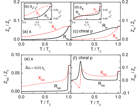
FIG. 3 (color online). Local impedance at a surface of the normal metal (i.e., x = -L ) versus temperature at \hbar\omega = 0.01\Delta_0 for (a) s -wave, (b) d_{x^2-y^2} -wave, (c) chiral p -wave, and (d) p_x -wave symmetry. The impedance of a NS bilayer versus temperature for (e) s -wave and (f) chiral p -wave symmetry.
