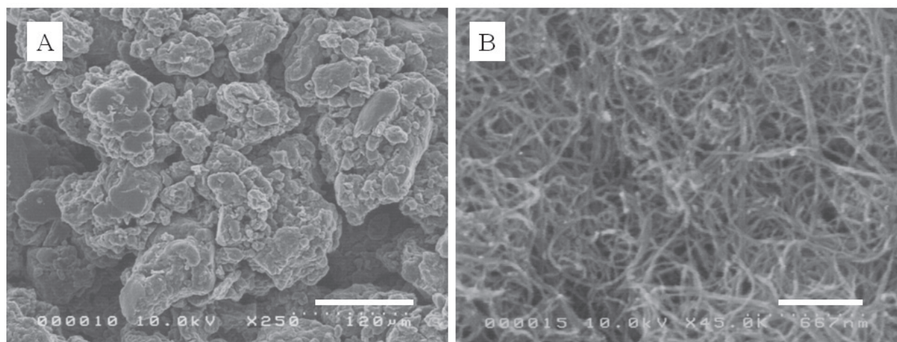
Fig. 1 SEM images of MWCNT used in the column chromatography at a lower magnification of \times 250 (A) where the bar indicates 0.1 mm, and at a higher magnification of \times 45,000 (B) where the bar indicates 500 nm.
