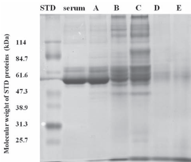
Fig. 3 SDS gel electrophoretic patterns of the chromatographic peaks in Fig. 2.
