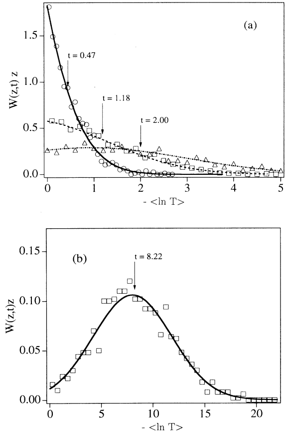
FIG. 6. Probability distribution of W(z, t) z vs -\ln T together with the numerical data for (a) extended phonons ( \langle T \rangle > T_{cr} = 0.26 ) with \langle T \rangle = 0.67 (solid line and circles), 0.42 (dashed line and squares), and critical states with \langle T \rangle = T_{cr} , i.e., L = \xi_{cr} (dot-dashed line and triangles), and for (b) localized phonons with \langle T \rangle = 0.02 (solid line and squares). The arrows indicate the positions of t = (-\ln T) . Note that z = 1/T . The numerical data are obtained for an ensemble of 1000 single-layer SL's by calculating T at a single frequency giving the chosen value of \langle T \rangle .
