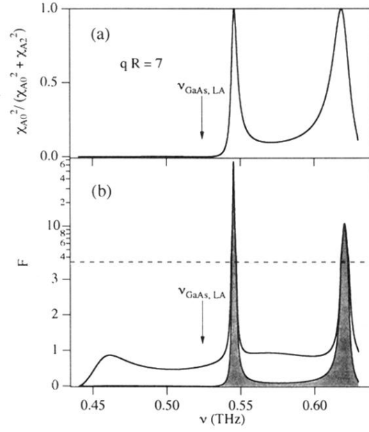
FIG. 7. (a) Contribution of the LA wave to the dilatational phonon mode versus frequency and (b) the corresponding F for R = 100 Å. The reduced longitudinal wave number is set at qR = 7 . The shaded region in (b) denotes the F solely attributed to the LA wave in the wire. The dashed horizontal line in (b) denotes the change of scale from a linear to a logarithmic one.
