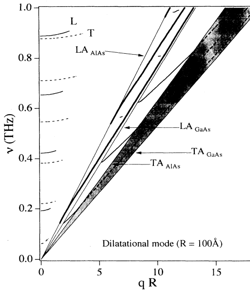
FIG. 8. Dispersions of the resonant dilatational phonon modes for R = 100 \text{ Å} . The thick and thin solid lines in the frequency region qv_{\text{AlAs,TA}} < \omega < qv_{\text{AlAs,LA}} denote the quasiconfined and entirely extended resonant modes, respectively. The dashed lines in the shaded region between the bulk-TA GaAs and TA AlAs dispersion curves are the dispersions of the confined dilatational modes (Ref. 31). The solid ( L ) and dashed ( T ) lines in the region \omega > qv_{\text{AlAs,LA}} are the dispersions of the entirely extended resonant modes attributed solely to the LA wave and TA wave in the wire, respectively.
