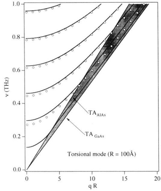
FIG. 4. Dispersions of the resonant torsional modes for R = 100 \text{ \AA} . The thick solid lines denote the dispersions and the thin lines in the shaded region between the bulk- \text{TA}_{\text{GaAs}} and -\text{TA}_{\text{AlAs}} dispersion curves are those of the confined torsional phonon mode (Ref. 31). The open circles denote the dispersions of the torsional phonon mode of a free-standing wire with the same radius.
