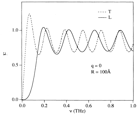
FIG. 9. Ratio F of the dilatational phonon modes versus frequency for R = 100 \text{ Å} in the region \omega > qv_{\text{AlAs,LA}} . The solid and dashed lines in the region \omega > qv_{\text{AlAs,LA}} are the dispersions of the resonant modes solely due to the LA wave and TA wave in the wire, respectively. The longitudinal wave number is taken as q = 0 .
