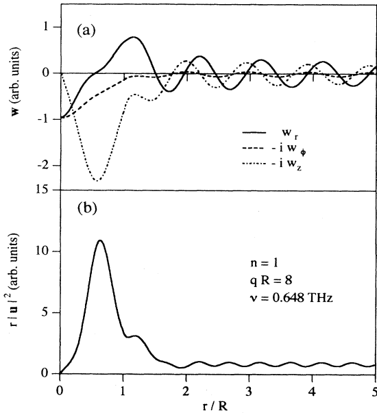
FIG. 10. (a) The radial, axial, and azimuthal components of amplitude w of the flexural phonon mode with n = 1 at \nu = 0.648 THz and qR = 8 for R = 100 Å and (b) the corresponding r|u|^2 versus r in the radial direction. The amplitude in the wire is found to be extremely enlarged in comparison with that in the surrounding medium.
