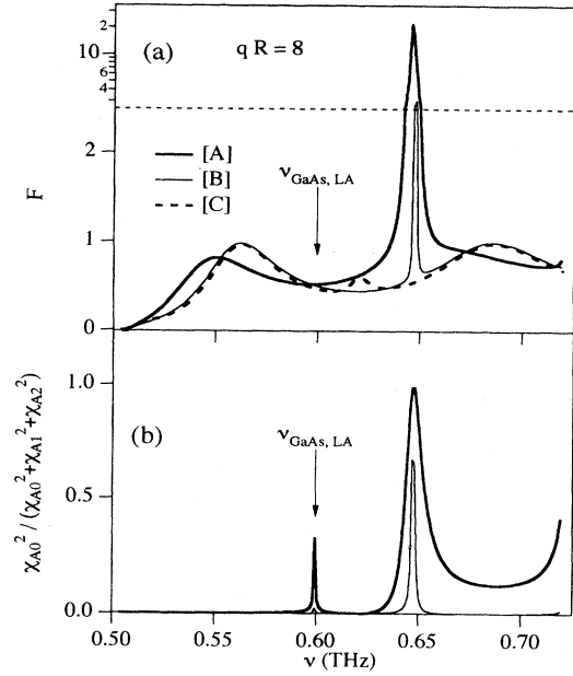
FIG. 11. (a) Ratio F of the flexural phonon mode with n = 1 versus frequency for R = 100 Å in the frequency region q v_{\text{AlAs,TA}} < \omega < q v_{\text{AlAs,LA}} and (b) the corresponding contribution of the LA wave to the flexural phonon at qR = 8 . The thick solid, thin solid, and dashed lines correspond to cases [A], [B], and [C] discussed in the text, respectively. The dashed horizontal line in (a) denotes the change of scale from a linear to a logarithmic one.
