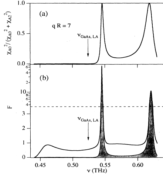
FIG. 7. (a) Contribution of the LA wave to the dilatational phonon mode versus frequency and (b) the corresponding F for R = 100 Å. The reduced longitudinal wave number is set at qR = 7 . The shaded region in (b) denotes the F solely attributed to the LA wave in the wire. The dashed horizontal line in (b) denotes the change of scale from a linear to a logarithmic one.
