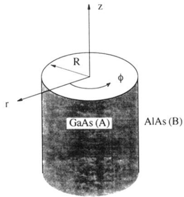
FIG. 1. Geometry of a cylindrical GaAs quantum wire surrounded by bulk AlAs.
