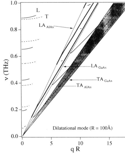
FIG. 8. Dispersions of the resonant dilatational phonon modes for R = 100 \text{ \AA} . The thick and thin solid lines in the frequency region qv_{\text{AlAs,TA}} < \omega < qv_{\text{AlAs,LA}} denote the quasiconfined and entirely extended resonant modes, respectively. The dashed lines in the shaded region between the bulk- \text{TA}_{\text{GaAs}} and \text{TA}_{\text{AlAs}} dispersion curves are the dispersions of the confined dilatational modes (Ref. 31). The solid ( L ) and dashed ( T ) lines in the region \omega > qv_{\text{AlAs,LA}} are the dispersions of the entirely extended resonant modes attributed solely to the LA wave and TA wave in the wire, respectively.
