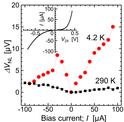
FIG. 2. (Color online) Bias-current dependence of \Delta V_{\text{NL}} measured at both 4.2 K and 290 K for a \text{Co}_{50}\text{Fe}_{50}/n\text{-GaAs} junction. Inset shows current-voltage characteristics of the Schottky junction of contact-2 measured at 4.2 K.
