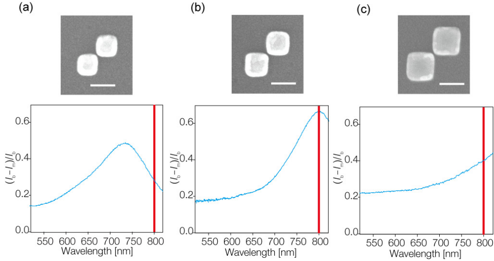
Fig. 4. SEM images of single gold nanoblock pairs with 5-nm gaps (top) and extinction spectra from arrays of the nanoblock pairs (longitudinal polarization) immersed in water (bottom). Nanoblock sizes: (a) 70 nm \times 70 nm \times 40 nm, (b) 80 nm \times 80 nm \times 40 nm, (c) 100 nm \times 100 nm \times 40 nm. Scale bar = 100 nm. The vertical red line in the spectra gives the incident laser wavelength.
