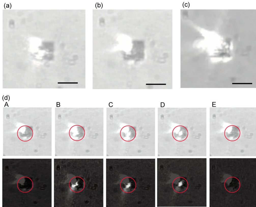
Fig. 5. Optical plasmonic trapping of 350-nm polystyrene particles with nanoblock pairs at the incident laser power of 15-μW. Block sizes: (a) (Media 1) 70 nm × 70 nm × 40 nm, (b) (Media 2) 80 nm × 80 nm × 40 nm, (c) (Media 3) 100 nm × 100 nm × 40 nm. Scale bar = 3 μm. (d) Top: Snapshots taken from (b) (Media 2) at several times: (A) 0.5 s, (B) 1.0 s, (C) 6.0 s, (D) 14.0 s, and (E) 15.0 s. Bottom: Images obtained by subtracting the first frame of the movie from each snapshot. The plasmonic trapping takes place in the red cycles of (d). Bright scattered light is observed around pairs. When nanoparticles pass sufficiently close to pairs, they get trapped and appear as bright scattering centers.
