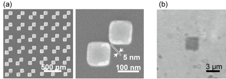
Fig. 2. (a) SEM and (b) transmitted images of an array of pairs of gold nanoblocks with 5-nm gaps. The right side of panel (a) shows a single nanoblock pair.
