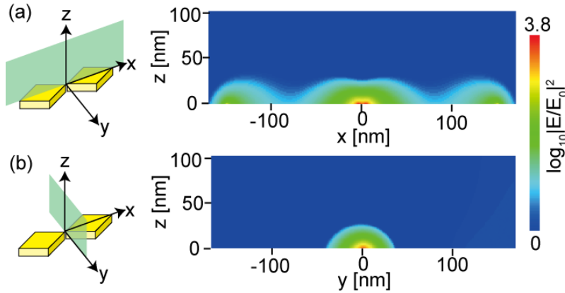
Fig. 3. Calculated near-field distributions near a model gold nanoblock pair at an 800-nm incident wavelength. Block size = 80 nm × 80 nm × 30 nm and gap distance = 5 nm. (a) xz plane and (b) yz plane on the pair as shown to the left side of panels (a) and (b), respectively.
