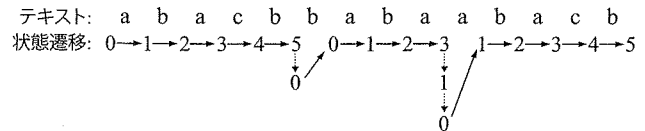
Fig. 3 KMP automaton for P = abacb .
