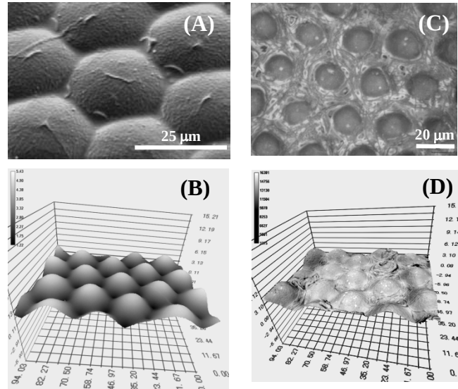
Figure 3. Images of agarose medium with a surface of concave type honeycomb (A, B) and honeycomb-patterned film with cellulose I polymorphism (C,D). A, SEM image; B, C and D, 3D-laser microscopic images, where B and D were magnified three times to height;
