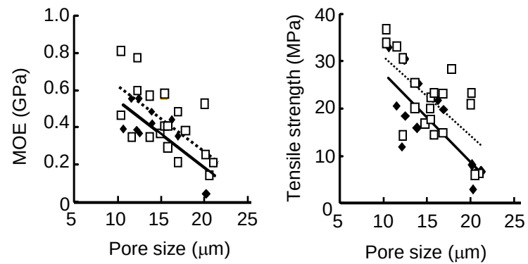
Figure 6. Effects of pore size of honeycomb-patterned film with cellulose II polymorphism on MOE and tensile strength. ◆, without lignin deposition; □, with lignin deposition.
