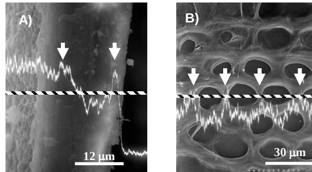
Figure 5. SEM images and bromine concentration in the cross section of AL- adsorbed flat bacterial cellulose film (A) and in the surface of AL-adsorbed honeycomb-patterned film with cellulose I polymorphism (B). The lines in the images show the scanning area of bromine by EDX. The arrows show the high concentration area of bromine.
