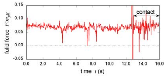
Fig. 11 Settling behavior and fluid force acting on a particle in assemblage. The pictures show at intervals of 2.0 seconds.
