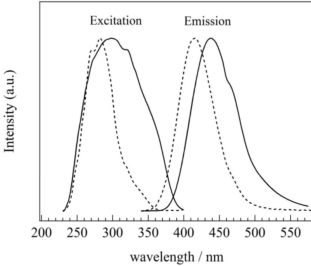
Figure 3 Emission and excitation spectra for MP-type \text{La}_{0.95}\text{Eu}_{0.05}\text{Al}_{12}(\text{O},\text{N})_{19} (solid lines) and \text{Ca}_{0.95}\text{Eu}_{0.05}\text{Al}_{12}\text{O}_{19} (broken lines). Emission spectra were measured under excitation at 254 nm and excitation spectra were monitored at 440 and 415 nm for \text{La}_{0.95}\text{Eu}_{0.05}\text{Al}_{12}(\text{O},\text{N})_{19} and \text{Ca}_{0.95}\text{Eu}_{0.05}\text{Al}_{12}\text{O}_{19} , respectively.
