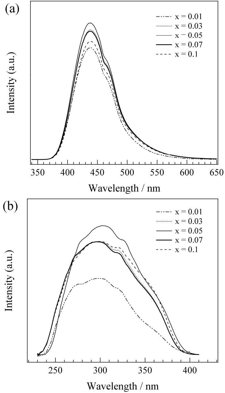
Figure 2 (a) Emission and (b) excitation spectra for MP-type \text{La}_{1-x}\text{Eu}_x\text{Al}_{12}(\text{O},\text{N})_{19} . Emission spectra were measured under excitation at 254 nm and excitation spectra were monitored at 440 nm.
