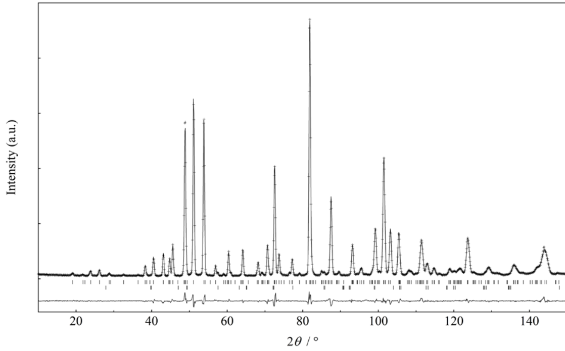
Figure 4 Observed (+), calculated (solid line) and difference powder neutron diffraction profiles for MP-type \text{La}_{0.97}\text{Eu}_{0.03}\text{Al}_{12}(\text{O},\text{N})_{19} . Upper vertical bars indicate the positions of Bragg reflections for the MP phase and the lower bars indicate those for \text{LaAlO}_3 (1 wt%).
