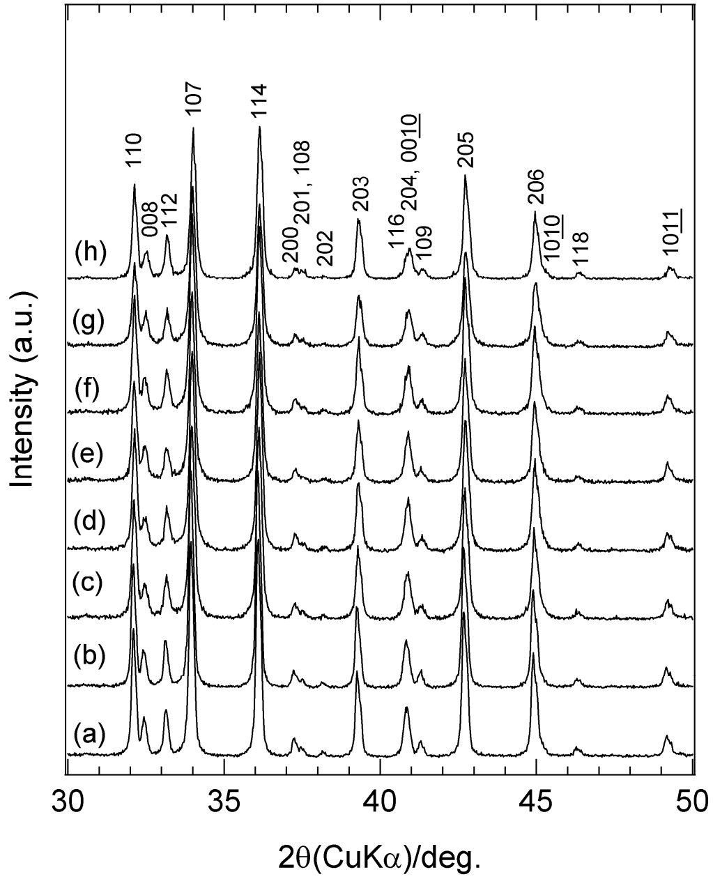
Figure 1 XRD patterns for MP-type \text{La}_{1-x}\text{Eu}_x\text{Al}_{12}(\text{O},\text{N})_{19} with various x ; (a) x = 0 , (b) x = 0.01 , (c) x = 0.03 , (d) x = 0.05 , (e) x = 0.07 , (f) x = 0.10 , (g) x = 0.20 , and (h) x = 0.30 .
