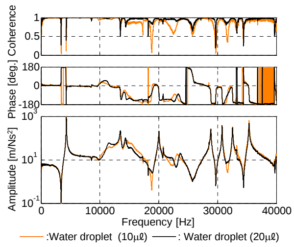
Fig.16 Auto-FRF H_{11} with water droplet 10μl and 20μl
