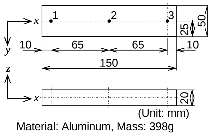
Fig. 4 Excitation and measurement points
