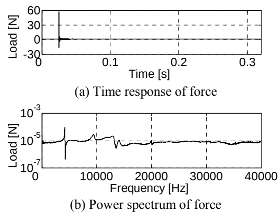
Fig. 6 Measured force by laser excitation
