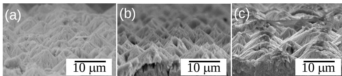
Fig. 7 Scanning electron micrographs of cross-sections of niobium specimens anodized at 10 V, following initial anodizing at 250 \text{ A m}^{-2} to 10 V, in glycerol electrolyte containing 0.6 \text{ mol dm}^{-3} \text{ K}_2\text{HPO}_4 and 0.2 \text{ mol dm}^{-3} \text{ K}_3\text{PO}_4 at (a) 433 K for 5.4 ks and immersing for 6.0 ks, (b) 443 K for 5.4 ks and (c) 453 K for 2.7 ks.
