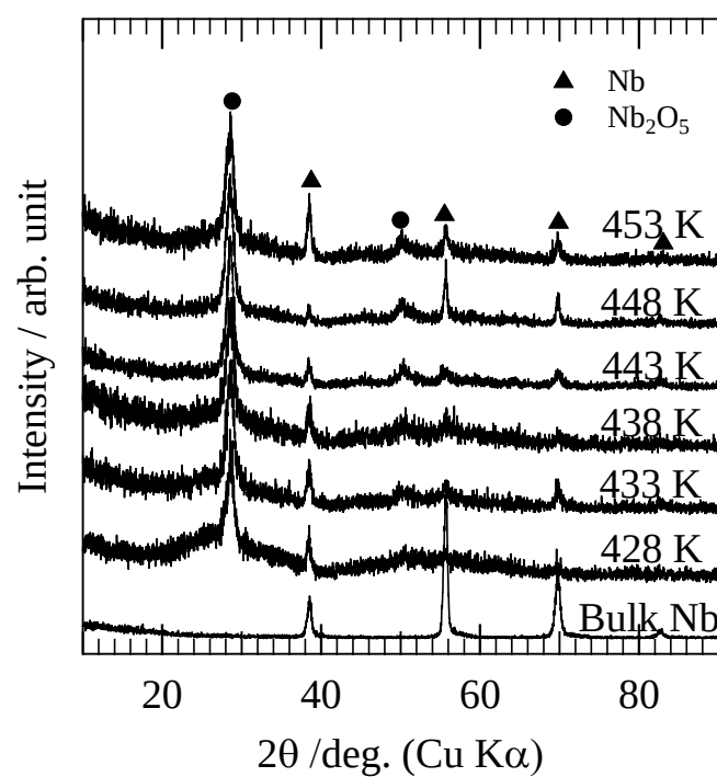
Fig. 2 X-ray diffraction patterns of niobium anodized at 10 V, following initial anodizing at 250 A m -2 to 10 V, in glycerol electrolyte containing 0.6 mol dm -3 K 2 HPO 4 and 0.2 mol dm -3 K 3 PO 4 for 5.4 ks at several temperatures.
