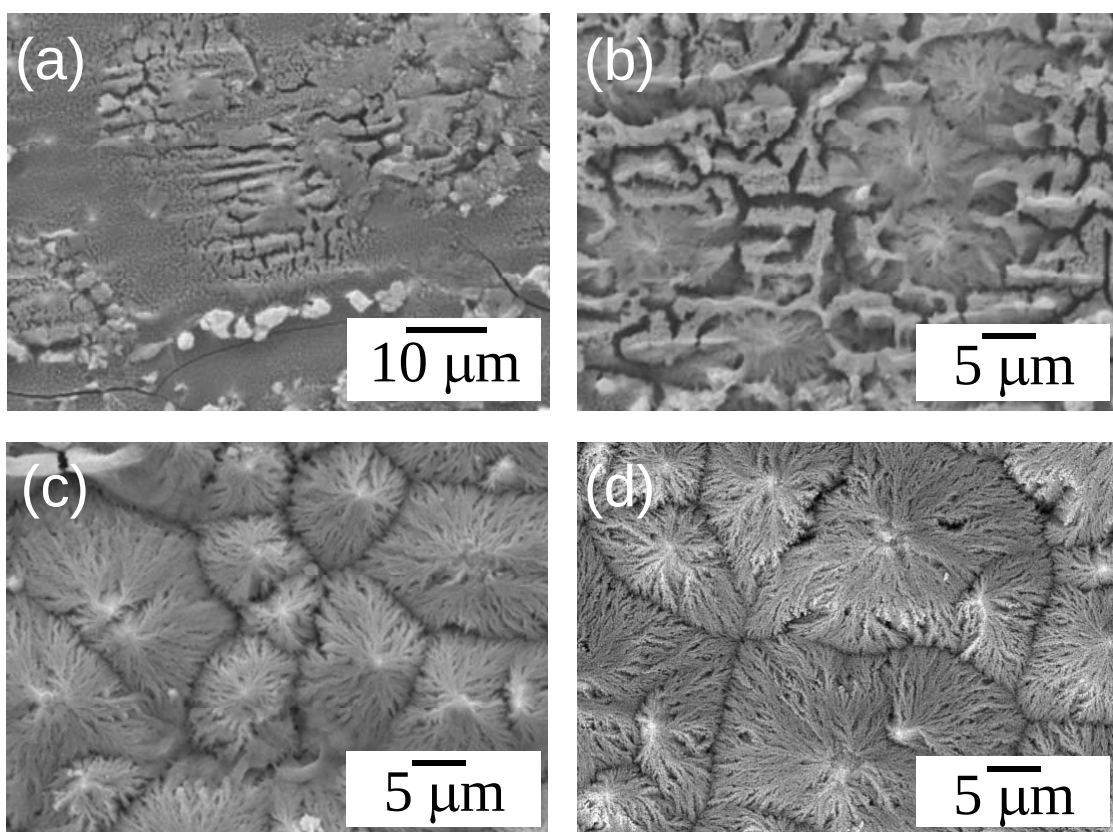
Fig. 5 Scanning electron micrographs of surfaces of niobium specimens anodized at 10 V, following initial anodizing at 250 \text{ A m}^{-2} to 10 V, in glycerol electrolyte containing 0.6 \text{ mol dm}^{-3} \text{ K}_2\text{HPO}_4 and 0.2 \text{ mol dm}^{-3} \text{ K}_3\text{PO}_4 for 5.4 ks at 433 K and then immersed in the same electrolyte for (a) 0 s, (b) 1.8 ks and (c) 3.6 ks at 433 K and (d) for 1.8 ks at 443 K.
