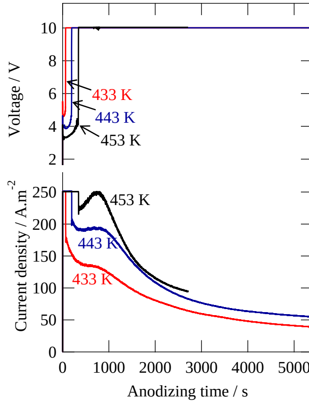
Fig. 1 Current-time and voltage-time responses of niobium during anodizing at 10 V in glycerol electrolyte containing 0.6 \text{ mol dm}^{-3} \text{ K}_2\text{HPO}_4 and 0.2 \text{ mol dm}^{-3} \text{ K}_3\text{PO}_4 at 433, 443 and 453 K. Initially, a constant current density of 250 \text{ A m}^{-2} was applied before reaching 10 V.
