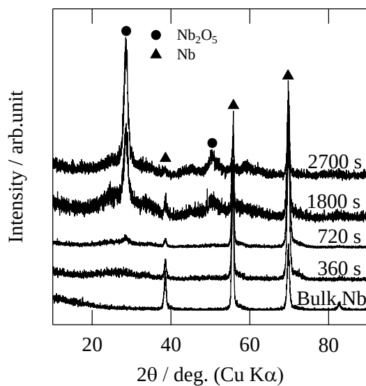
Fig. 3 X-ray diffraction patterns of niobium anodized at 10 V, following initial anodizing at 250 \text{ A m}^{-2} to 10 V, in glycerol electrolyte containing 0.6 \text{ mol dm}^{-3} \text{ K}_2\text{HPO}_4 and 0.2 \text{ mol dm}^{-3} \text{ K}_3\text{PO}_4 for several periods of time at (a) 433 K, (b) 443 K and (c) 453 K.
