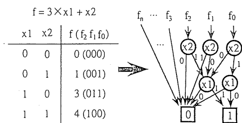
Fig. 9 BDD representation for B-to-I functions.
