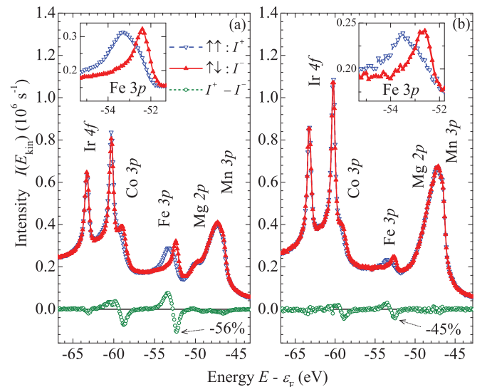
FIG. 7. (Color online) MCDAD for the shallow core level spectra obtained from the buried CoFe on top and Co 2 FeAl beneath a 10-nm-thick IrMn film. The insets show an enlarged view of the Fe 3p states.
