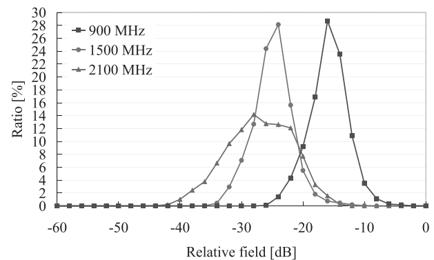
Fig. 11 E-field histograms of the region of interest.
