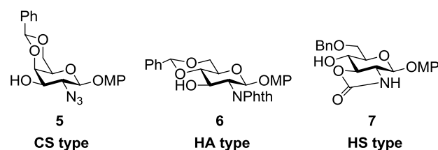
Figure 1. donors and acceptors employed in this study. MP: p -methoxy phenyl.
