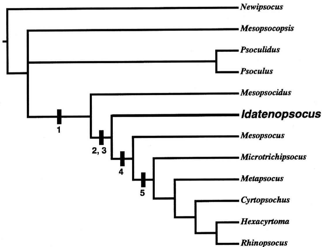
Fig. 5. Inferred phylogenetic position of Idatenopsocus orientalis in the family Mesopsocidae. Tree modified from Badonnel and Lienhard (1988). The numbered shaded squares indicate following apomorphic character states: 1, distinct neck at base of egg guide; 2, long anal vein in hindwing; 3, thickened wall of spermathecal sac; 4, loss of subapical placoid sensillum on 6th flagellar segment; 5, neoteny of female.
