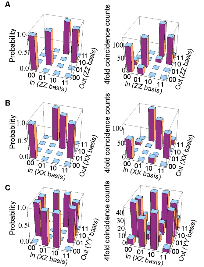
Fig. 3. Experimental demonstration of a KLM CNOT gate. Left: ideal operation. Right: fourfold coincidence count rates (per 5000 s) detected at DC , DT , DA1 and DA2 . (A) For control qubit, |0_Z\rangle = |V\rangle , |1_Z\rangle = |H\rangle ; for target qubit, |0_Z\rangle = 1/\sqrt{2}(|V\rangle + |H\rangle) , |1_Z\rangle = 1/\sqrt{2}(|V\rangle - |H\rangle) . ‘10’ indicates C = 1 and T = 0 . (B) For control qubit, |0_X\rangle = 1/\sqrt{2}(|V\rangle + |H\rangle) , |1_X\rangle = 1/\sqrt{2}(|V\rangle - |H\rangle) ; for target qubit, |0_X\rangle = |V\rangle , |1_X\rangle = |H\rangle . (C) For control qubit, |0_Y\rangle = 1/\sqrt{2}(|V\rangle + i|H\rangle) , |1_Y\rangle = 1/\sqrt{2}(|V\rangle - i|H\rangle) ; for target qubit, |0_Y\rangle = 1/\sqrt{2}(|V\rangle - i|H\rangle) , |1_Y\rangle = 1/\sqrt{2}(|V\rangle + i|H\rangle) . The events in which two pairs of photons are simultaneously incident to the ancillary inputs and no photons are incident to the signal inputs are subtracted, as confirmed by a reference experiment without input photons
