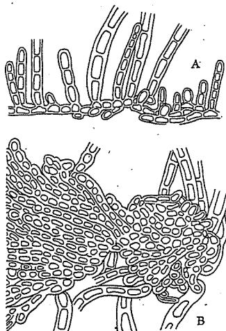
Fig. 6. R. plumosum DREW. A. Basal parts in transverse section. \times 250 . B. Basal parts seen from below. \times 250 .
