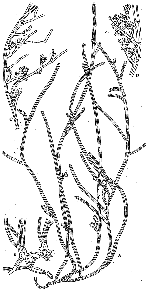
Fig. 8. R. callithamnoides NAKAMURA. A. Plant with monosporangia. \times 140 . B. Basal parts. \times 223 . C. Branch with antheridial branchlets and one monosporangium. \times 166 . D. Branch with antheridial branchlets showing their arrangement. \times 250 .
