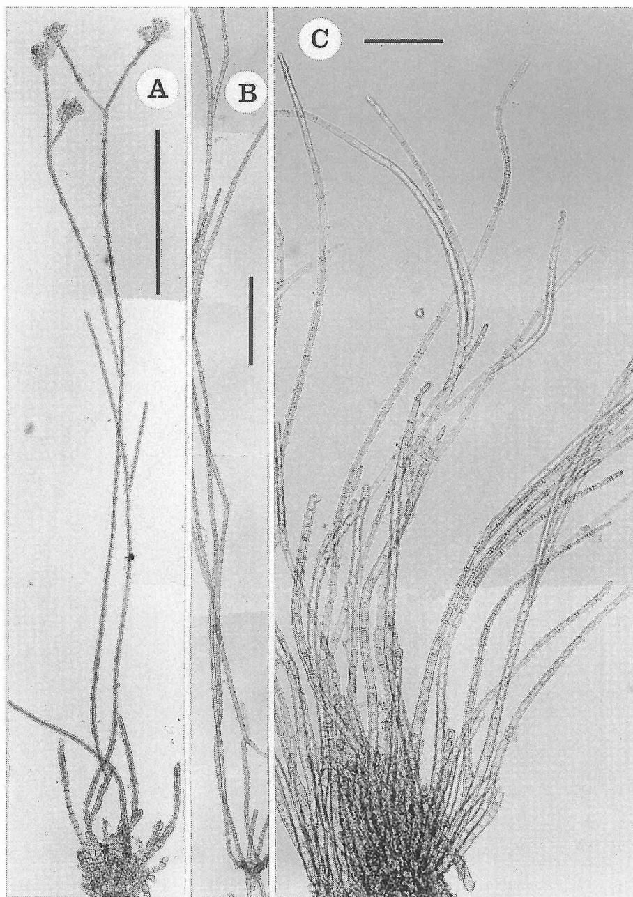
Fig. 16. Rhodochorton purpureum . A: Thallus of Oshoro 2 strain. B: Thallus of Nemuro strain. C: Thallus of Akkeshi strain. (Scale bar of Fig. A is 500 \mu m. Scale bar of Fig. B is 300 \mu m. Scale bar of Fig. C is 100 \mu m.)
