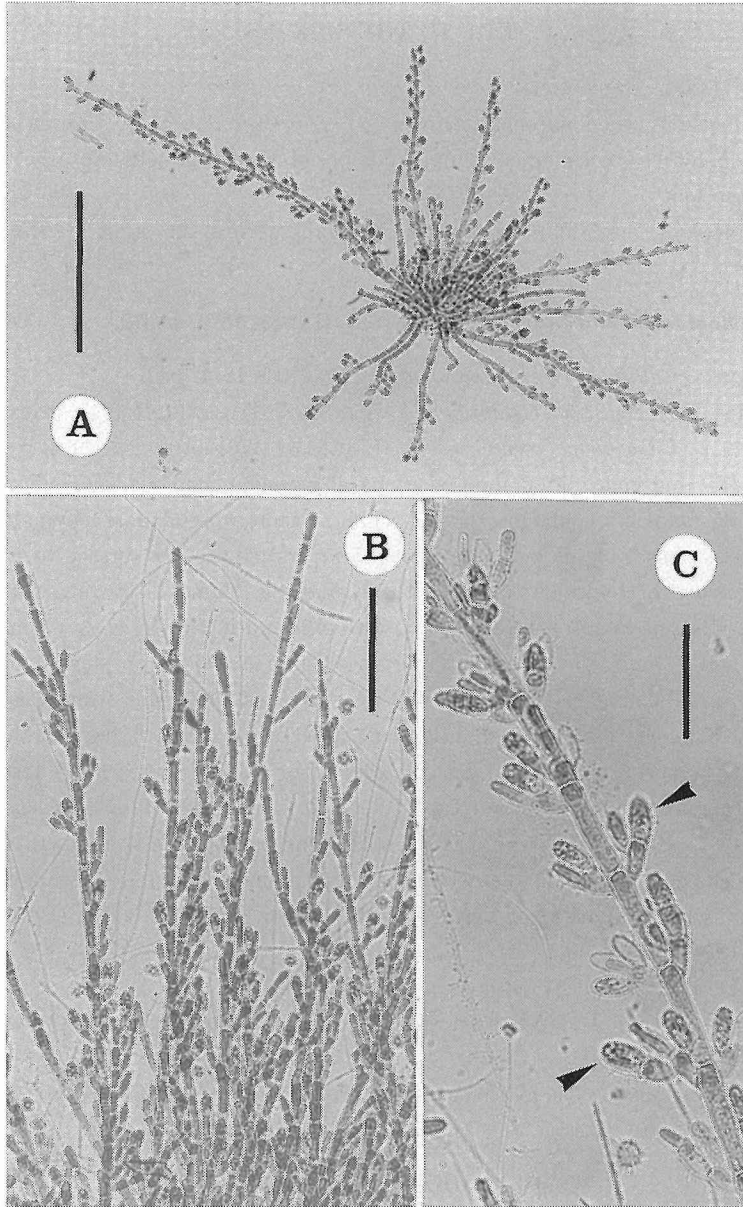
Fig. 13. Acrochaetium strictum . A: A plant in culture. Note simple and straight form of erect filaments. B: Erect filaments in culture. C: Monosporangia (arrow heads) born solitarily or in pairs on a stalk cell. (Scale bar of Fig. A is 200µm. Scale bar of Fig. B is 100µm. Scale bar of Fig. C is 50µm.)
