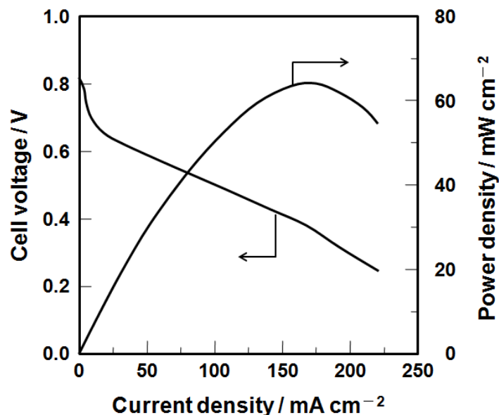
Figure 3 Performance of direct-ethanol solid alkaline inorganic fuel cell testing Anode, Fe-Co-Ni; electrolyte: \text{NaCo}_2\text{O}_4 ; cathode: catalyst free; Cell Temp., 80^\circ\text{C} ; Anode gas, 20-mL flow of ethanol/ \text{He}+\text{N}_2 ; Cathode gas, 20-mL flow of \text{H}_2\text{O} -
