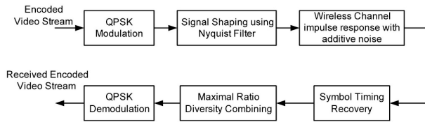
Fig. 10 Block diagram of wireless video transmission system.
