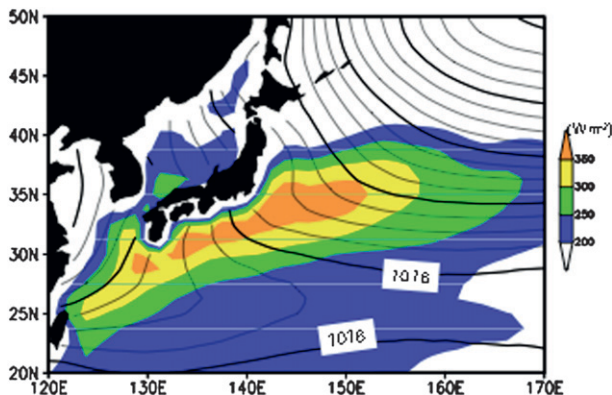
FIG. 9. Winter climatology of SLP (contours; CI = 1 hPa) and Q (colors; \text{W m}^{-2} ) based on JRA-25. Shading convention and scale of arrows are given to the right of each panel.
