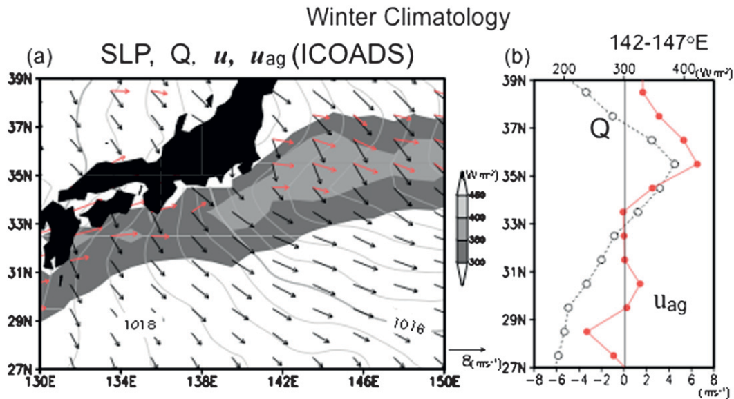
FIG. 4. (a) Winter climatology of surface wind (black arrows; \text{m s}^{-1} ), and ageostrophic wind (red arrows; \text{m s}^{-1} ), superimposed on SLP (gray contours; \text{CI} = 0.5 \text{ hPa} ), and Q (gray shades; \text{W m}^{-2} ) based on ICOADS. Ageostrophic winds less than 3.5 \text{ m s}^{-1} are not represented. Shading convention and scale of arrows are represented to the right. (b) Climatological meridional plots of winter means in ageostrophic zonal winds (solid red; \text{m s}^{-1} ) and Q (dashed black; \text{W m}^{-2} ) averaged over 142^{\circ}\text{--}147^{\circ}\text{E} based on ICOADS. Note that the axis for Q is at the top of the panel, but the axis for the ageostrophic zonal winds is at the bottom of the panel.
