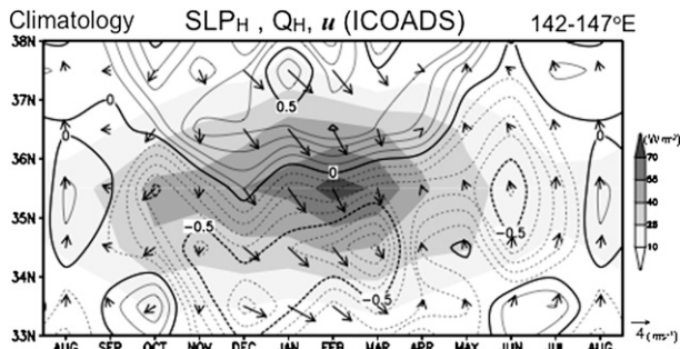
FIG. 8. Climatological seasonal cycle of high-pass-filtered SLP (contours; CI = 0.1 hPa) and Q (gray shades; \text{W m}^{-2} ) and surface wind vectors (arrows; \text{m s}^{-1} ) averaged over 142^{\circ} – 147^{\circ}\text{E} , based on ICOADS. Negative values are dashed. Note that the horizontal axis begins and ends in August. Shading convention and scale of arrows are given to the right.
