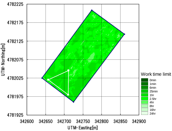
Fig. 18 GIS map of work time limit for vibration acceleration in the vertical direction ( a_z ).
