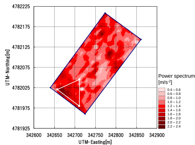
Fig. 12 GIS map of the maximum vibration acceleration in the lateral direction ( a_y ) for 1–10 Hz.
