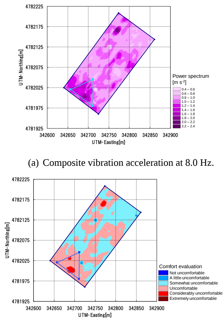
(b) Comfort evaluation using the composite vibration acceleration at 8.0 Hz. Fig. 20 GIS map of composite vibration acceleration at the 1/3 octave band center frequency of 8.0 Hz and a comfort evaluation.
