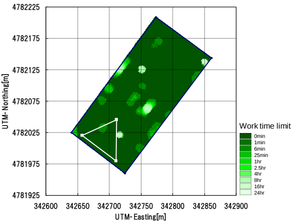
Fig. 10 GIS map of work time limit for vibration acceleration in the longitudinal direction ( a_x ).
