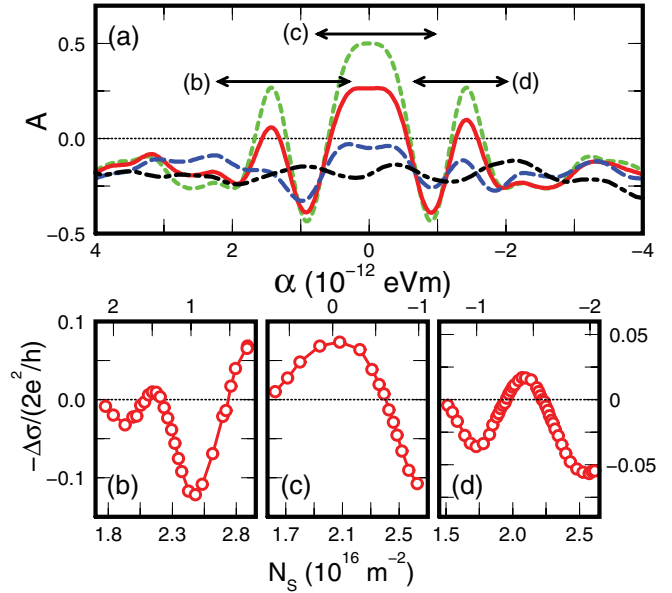
FIG. 2. (Color online) (a) Simulated spin interference (SI) patterns for the 2D-extended structure shown in Fig. 1. The dashed (green), solid (red), long-dashed (blue), and dash-dotted (black) curves denote the results with \gamma = 0, 4, 8 , and 27 \text{ eV \AA}^3 , respectively. The parts that reproduce the experiments shown in (b)–(d) are indicated by the horizontal bars with arrows at both ends. (b)–(d) Experimental SI patterns with L = 1.8 \mu\text{m} (Ref. 9). The epiwafers used in (b)–(d) are, respectively, samples 2, 3, and 4 in Refs. 4 and 9. The ordinates for (b) and (c) are given on the left and that for (d) is given on the right side of the graphs. The approximate values of \alpha in (b)–(d) are given on the top scale linearly correlating \alpha with N_S .
