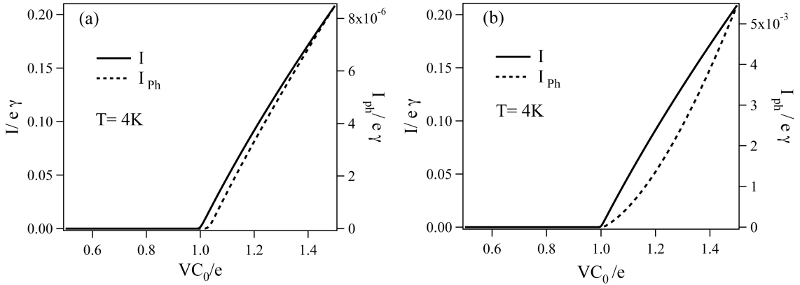
FIG.4: The total current I and phonon mediated current I_{\text{ph}} for (a) the breathing and (b) oblong modes versus V at 4 K .
