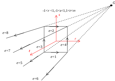
Fig. 1. Local coordinates of infinite element
