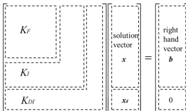
Fig. 2. Deflated full coefficient matrix
