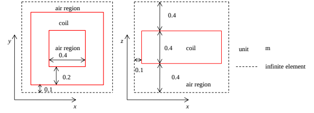
Fig. 3. Analysis coil model
