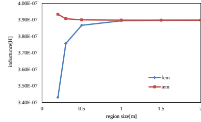
Fig. 5. influence of air region size on inductance
