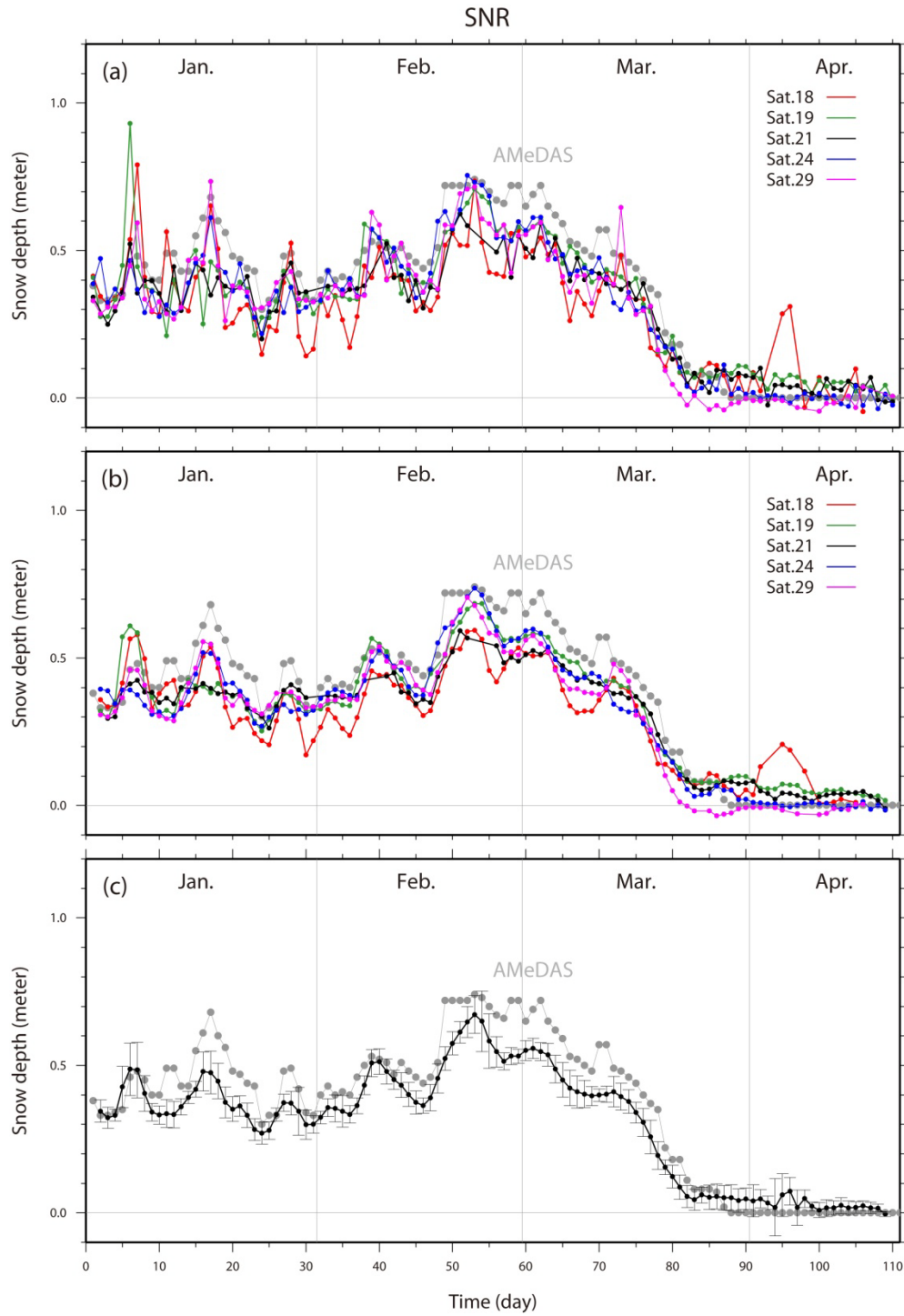
Figure 8. Snow depth time series obtained using SNR data from satellites 18, 19, 21, 24, and 29. See the caption of Fig. 7 for detail. The average of the standard deviation was \sim 0.041 m.
