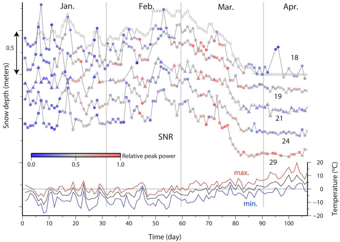
Figure 10. Snow depth estimated by analyzing the SNR data of the five satellites (whose numbers are attached to the right), with colors of symbols showing the relative strength of the peak. Individual time series are given vertical offset to facilitate visualization. At the bottom, we show daily average (black curve), maximum (red), and minimum (blue) temperature at the Shinshinotsu AMeDAS station.
