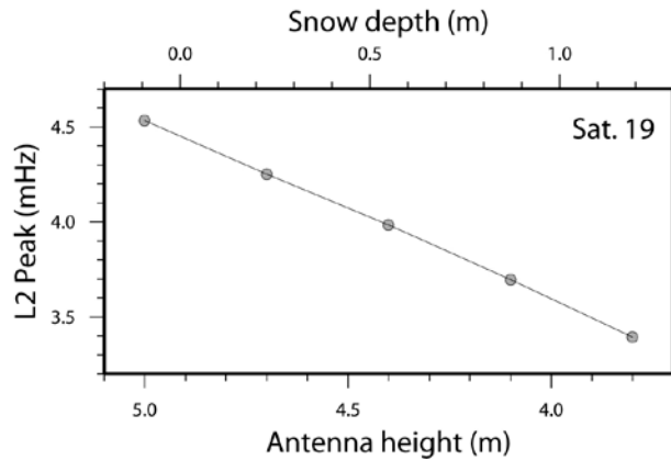
Figure. 3. Calibration curve to relate the L2 peak frequency to the snow depth inferred from synthesized multipath signatures as shown in Fig. 2a. The calibration equation is expressed as [Snow depth] (meter) = \{4.4 - [\text{Frequency peak}] (\text{mHz})\} / 0.93 . This curve is valid only for the ascending satellite 19 received at the Shinshinotsu GPS station.
