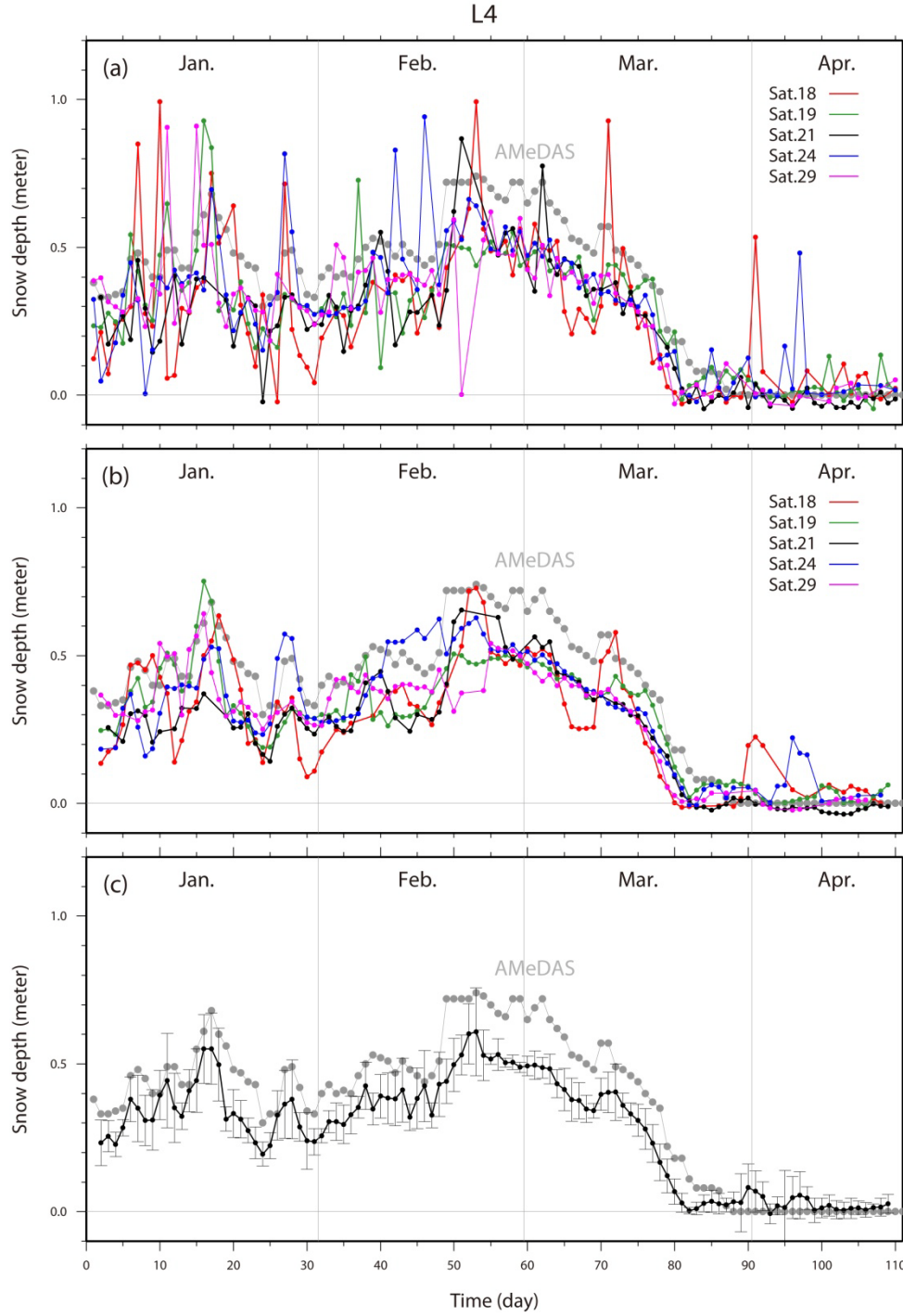
Figure. 7 (a) Raw snow depth time series obtained using L4 data from satellites 18, 19, 21, 24, and 29. The AMeDAS snow depth time series are shown with gray dots. (b) To reduce noise, spectrograms of the three consecutive days have been stacked to estimate the spectral peak of the middle day. (c) Daily averages of the snow depths by the five satellites in (b). The error bars show one standard deviation, and the average standard deviation was \sim 0.062 m. The whole time series is shifted negatively from AMeDAS by \sim 0.1 m.
