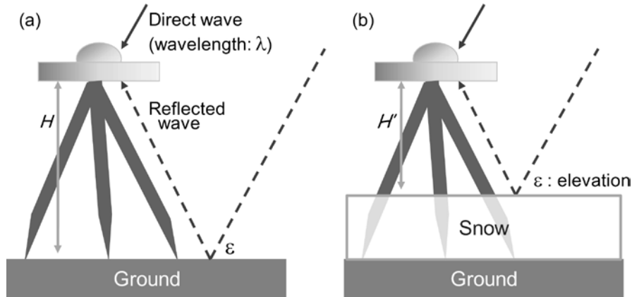
Figure. 1.(a) Multipath is the interference between the direct and reflected waves. The excess path length of the reflected wave changes as the satellite moves in the sky at a rate depending on the antenna height H , which decreases to H' as snow accumulates on the ground (b).
