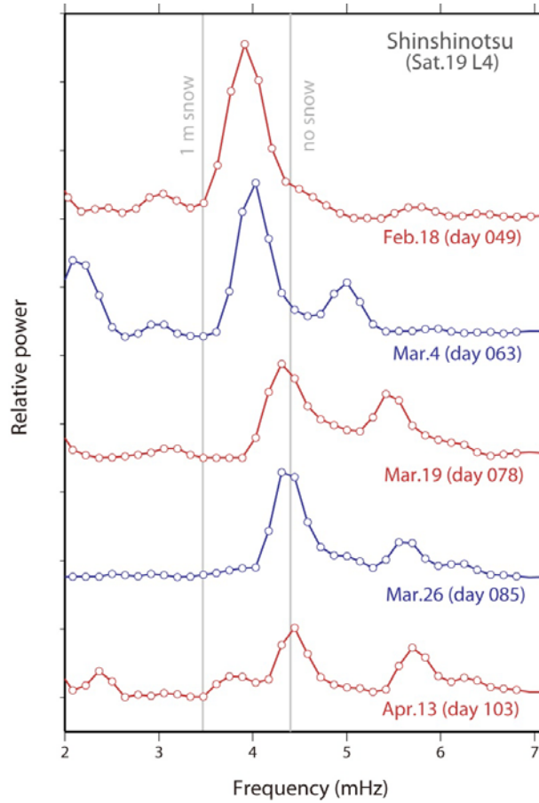
Figure. 6. The spectrograms of the L4 multipath signatures of the rising satellite 19 observed at the Shinshinotsu GPS station on five selected days from February to April, 2009. Positions of the peaks contain the information on the snow depths. The two gray vertical lines correspond to no snow and 1 meter snow.
