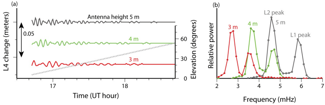
Figure. 2. (a) Temporal changes of the L4 phase (in meter) calculated for the first two hours after the rise of the satellite 19 on March 1, 2009, at the Shinshinotsu (020877) GPS station, using the equation (2) assuming three different heights of antenna (3, 4 and 5 m, which means snow depths of 2, 1, and 0 m because the original antenna height is 5 m). We calculated \alpha assuming 0.15 for the microwave reflectivity at the ground and the antenna pattern given in Bilich et al. (2008). The gray dotted line shows the change in the satellite elevation. (b) Spectrogram of the three L4 phase time series in (a) are composed of two distinct peaks originating from phase changes of L1 and L2. We use the L2 peak (the one with the lower frequency) to estimate snow depths.
