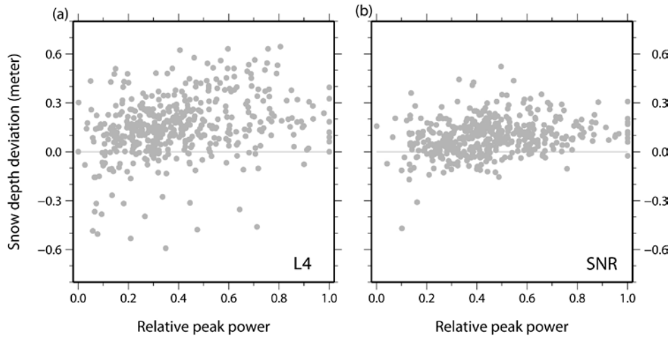
Figure 9 Relationship between relative peak power strength and the deviation of the snow depths (AMeDAS minus GPS) by L4 (a) and SNR (b). Peak power is taken relative to the day of the largest power for individual satellites.
