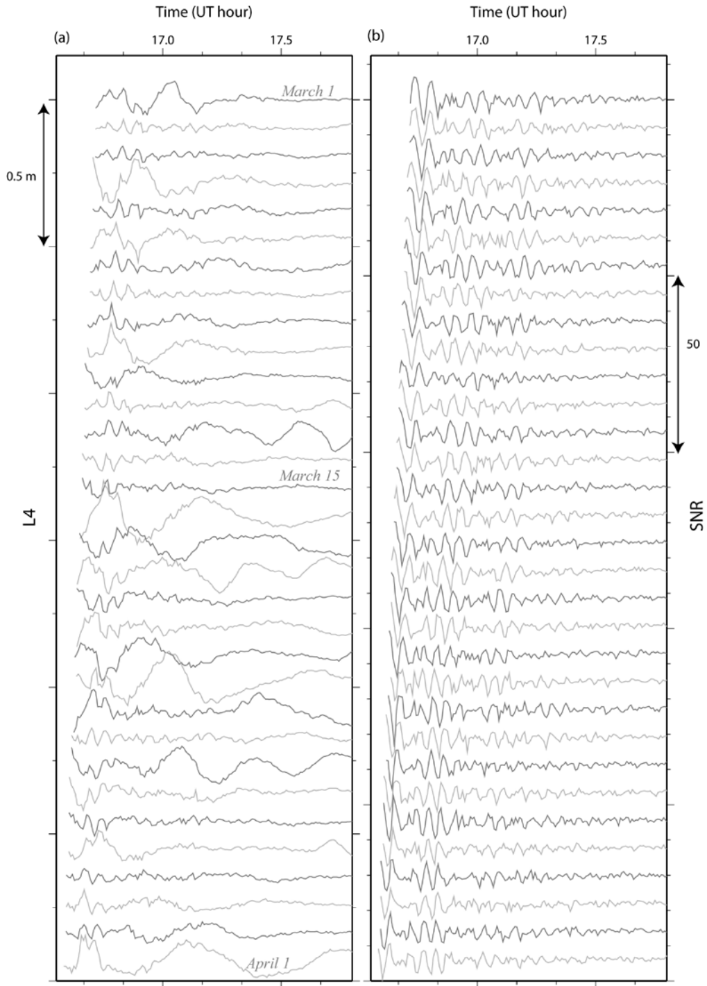
Figure. 5. The time series of L4 (a) and SNR (b) from 1 March to 1 April, 2009, of satellite 19 at the Shinshinotsu GPS station. The label of the horizontal axis at the top is valid only for the uppermost time series because the observing window is shifted \sim 4 minutes earlier per day to keep the same satellite positions in the sky.
